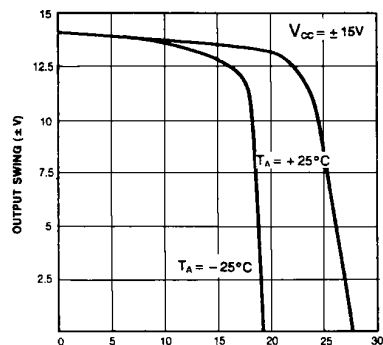
Figure 3. Current Limiting
