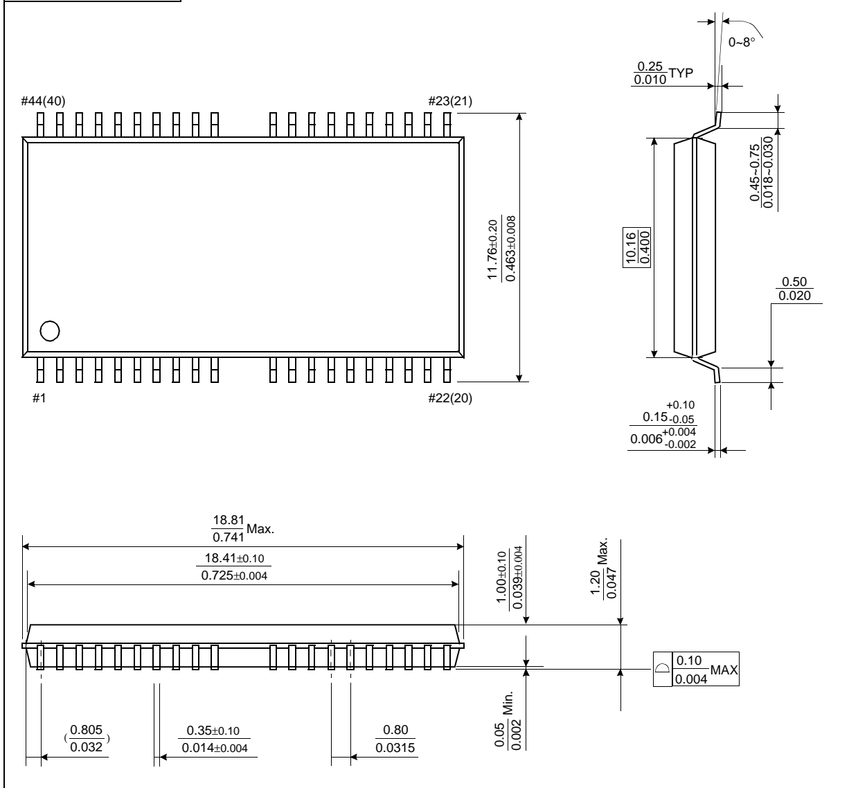
Unit :mm/Inch
