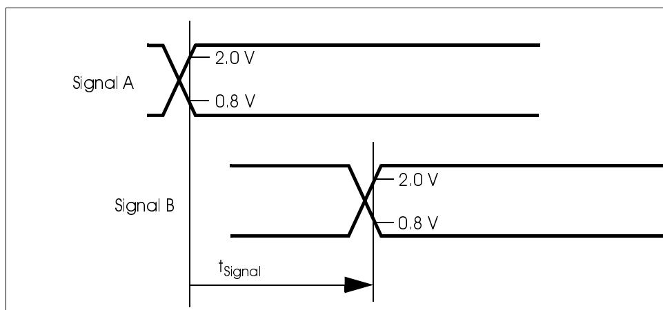
Figure 1-17: Asynchronous Signals
