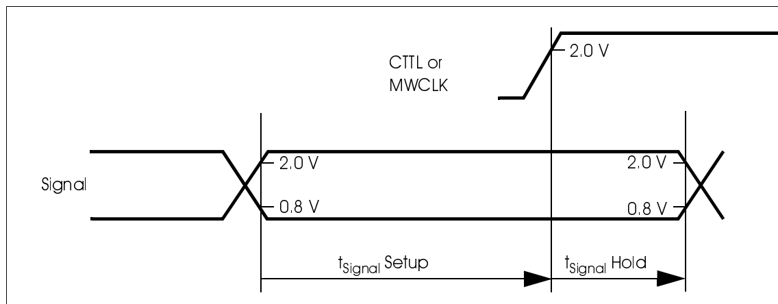
Figure 1-16: Synchronous Input Signals
