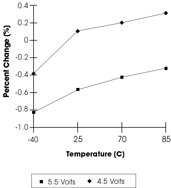
Chart 4: Oscillator Stability
