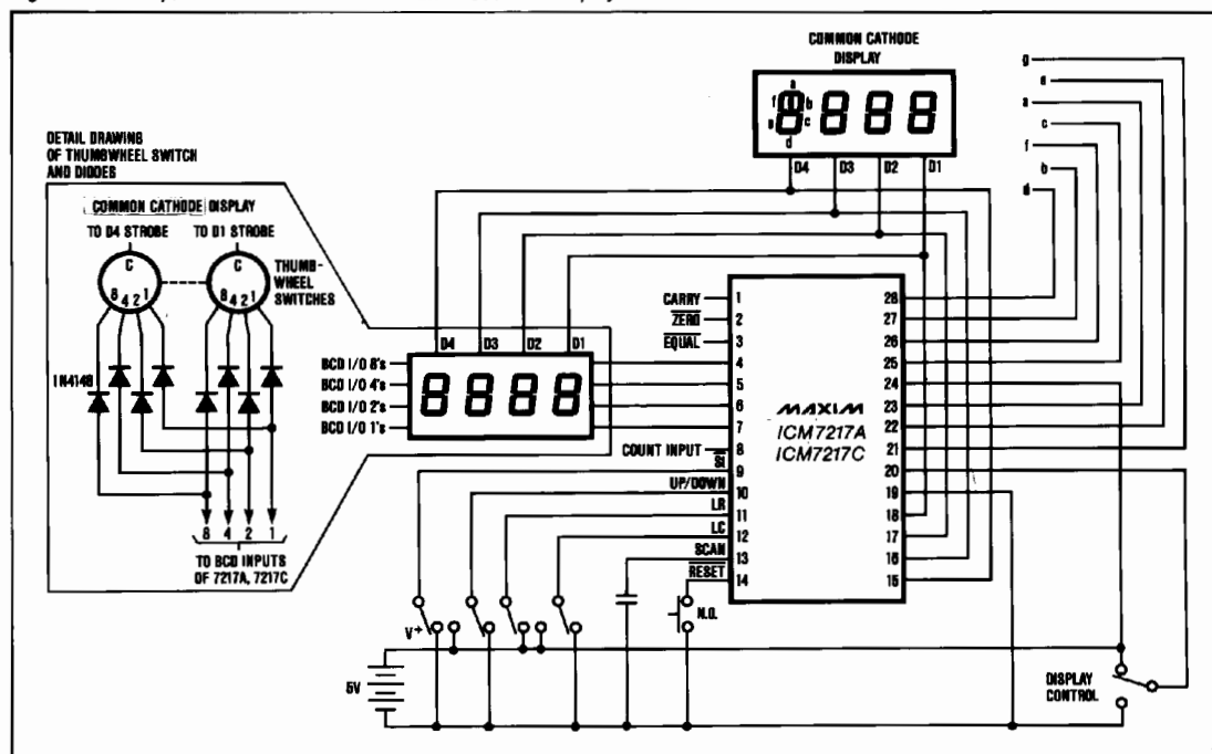
Figure 2. Basic Up/Down Counter with Common Cathode LED Display.
