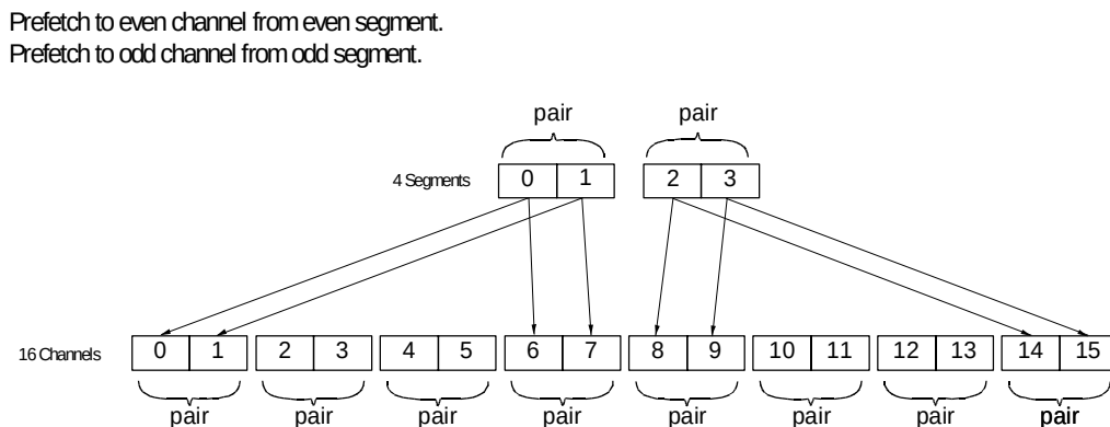
Figure 37 Pair Prefetch Operation Basics 1
