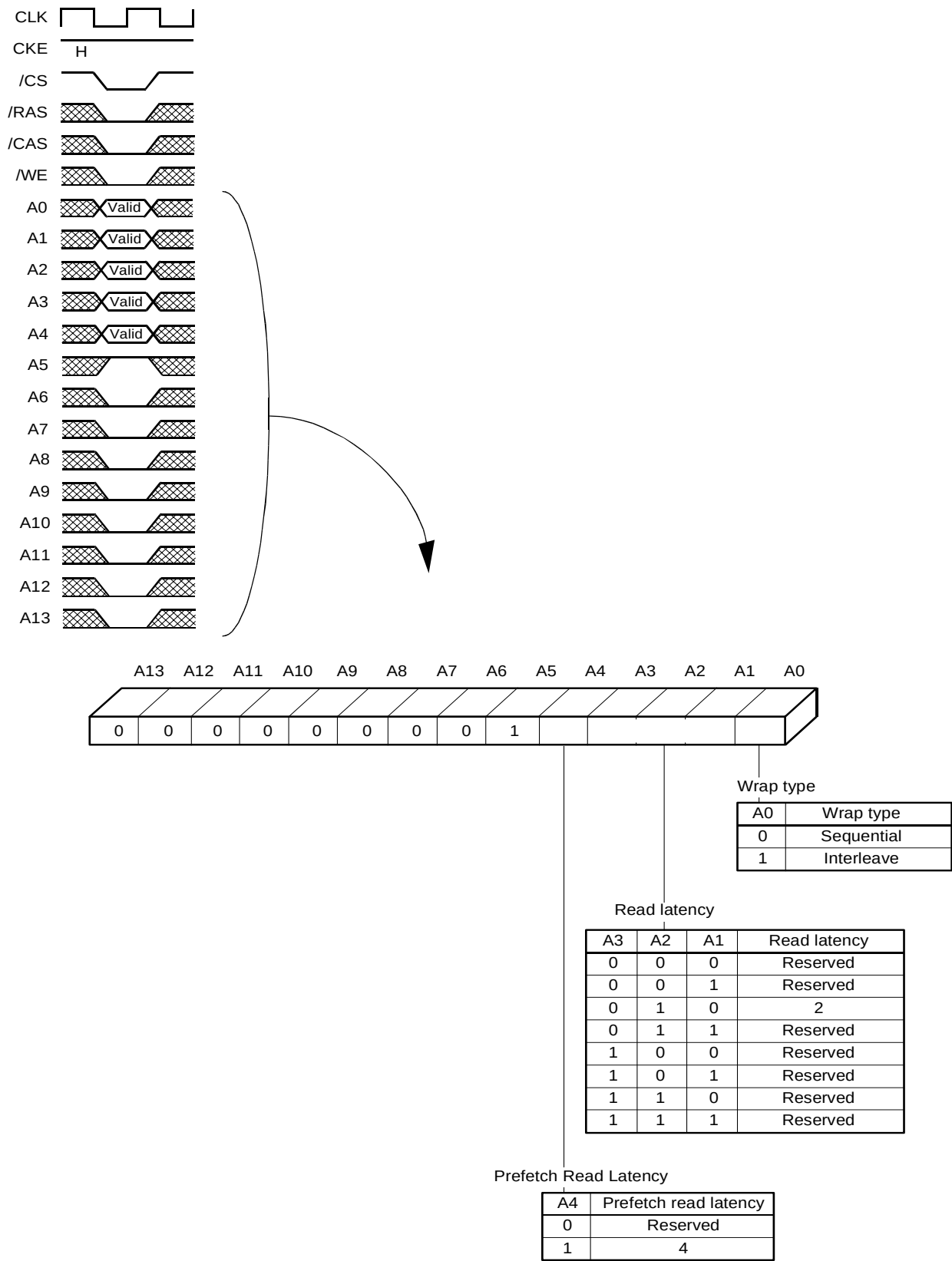
Figure 40 Channel Latency register
