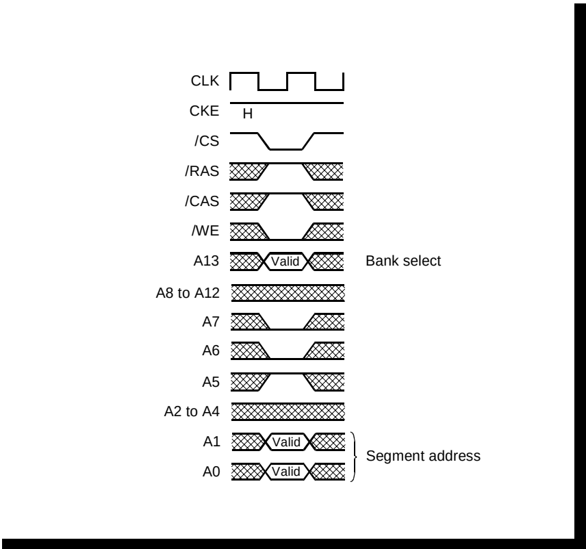
Figure 13 Prefetch to Dummy without Autoprecharge Timing
