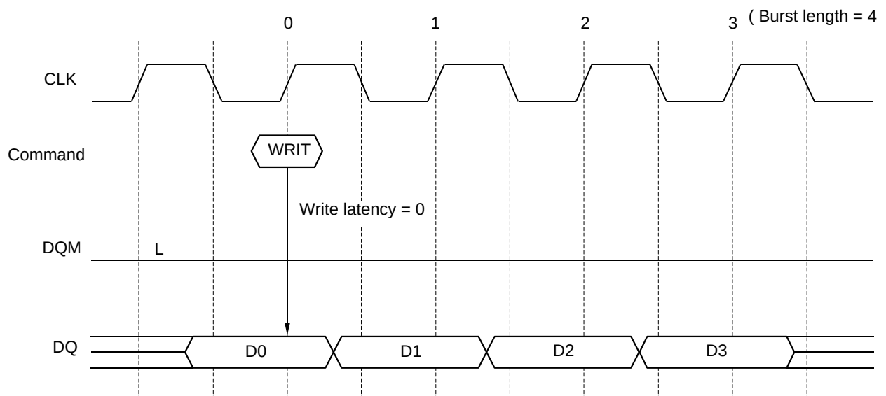
Figure 50 Write Operation
