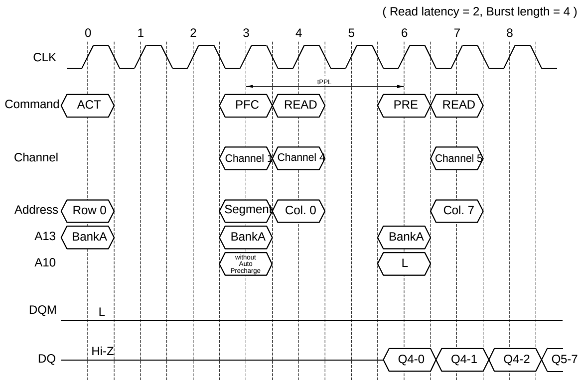
Figure 58 Prefetch to Read Operation without Auto Precharge (Other Channel Read)
