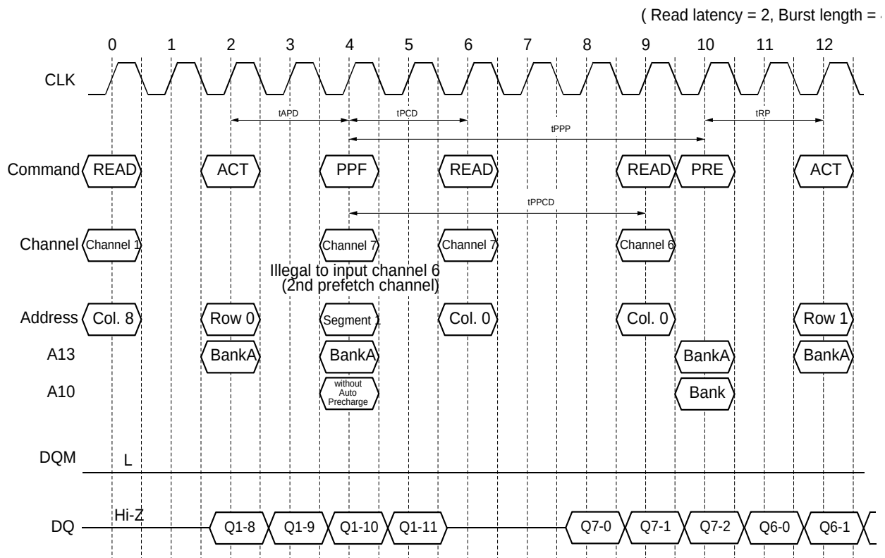
Figure 83 Pair Prefetch Operation
