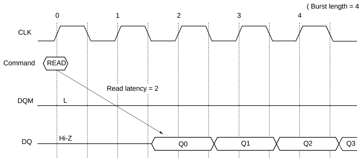
Figure 49 Read Operation
