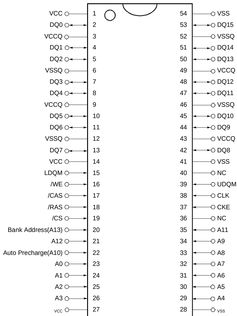
Figure 3 Pin Configuration HYB39V6416yT
