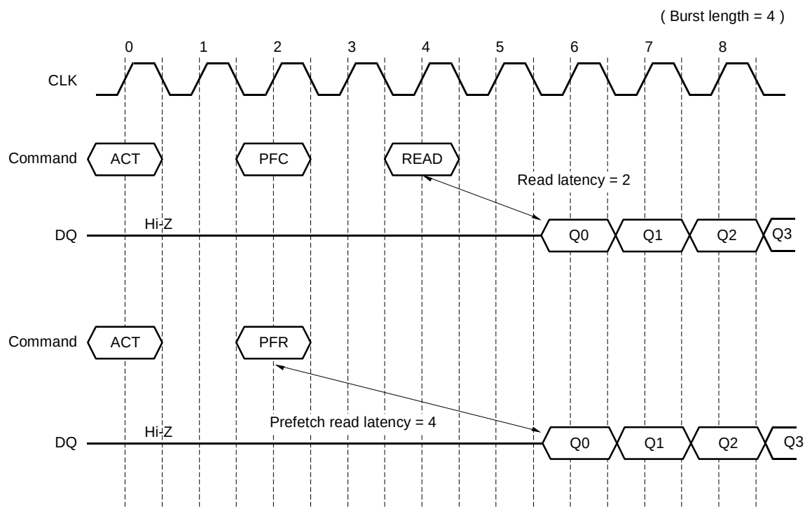
Figure 32 Prefetch Read Operation Timing
