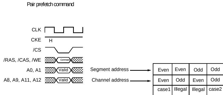
Figure 38 Pair Prefetch Operation Basics 2
