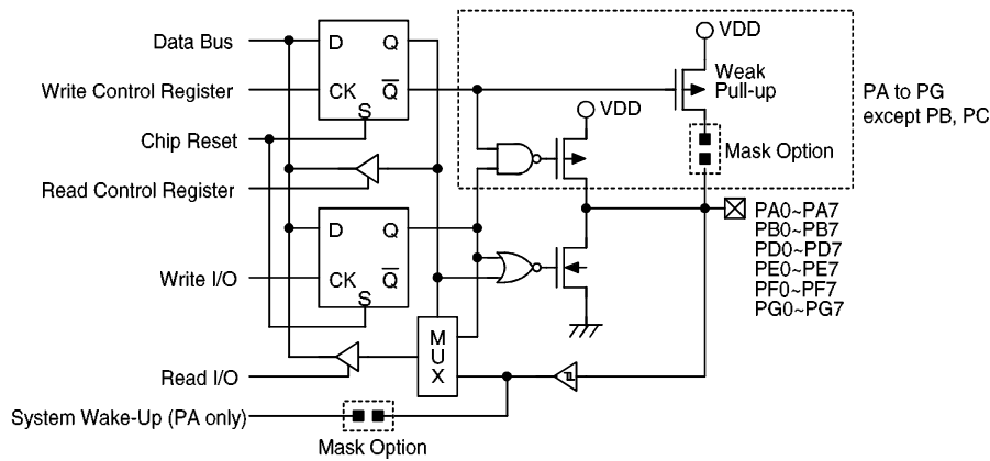
Input/output ports
