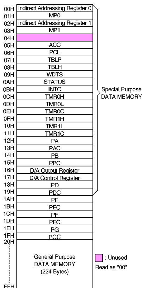
RAM mapping
