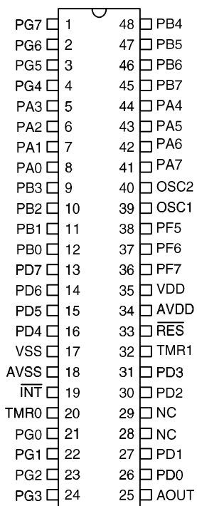
HT99C810/HT99C811 – 48 SSOP
