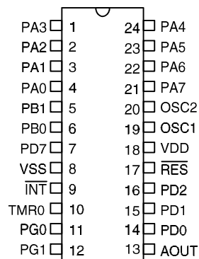
HT99C810/HT99C811 – 24 SDIP
