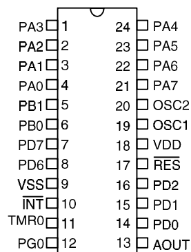
HT99C810/HT99C811 – 24 SOP
