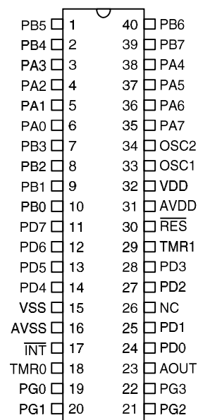
HT99C810/HT99C811 – 40 DIP
