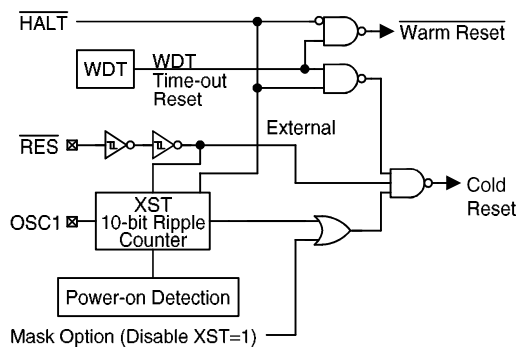
Reset configuration
