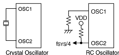
System oscillator
