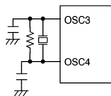
RTC oscillator
