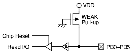
PB input lines
