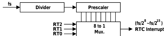
Real time clock
