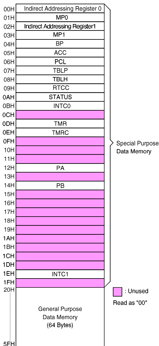
RAM mapping
