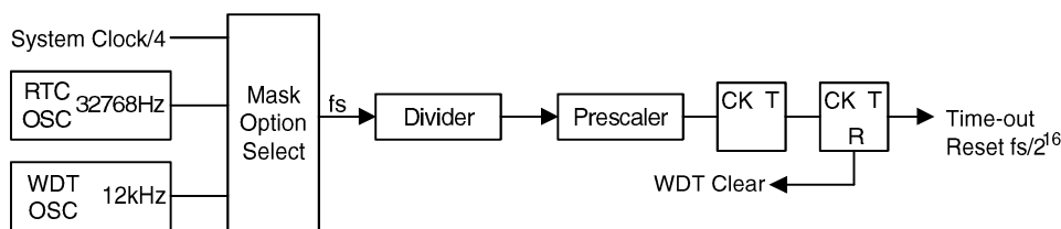
Watchdog timer
