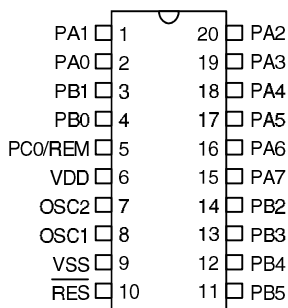
HT48RA0 - 20 DIP-A
