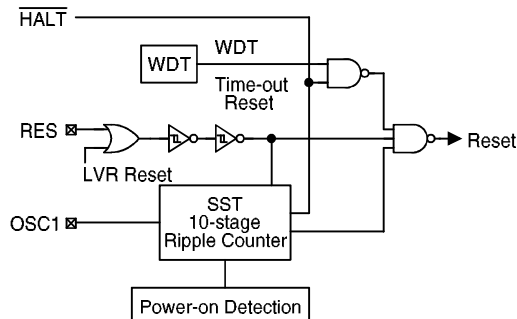
Reset configuration
