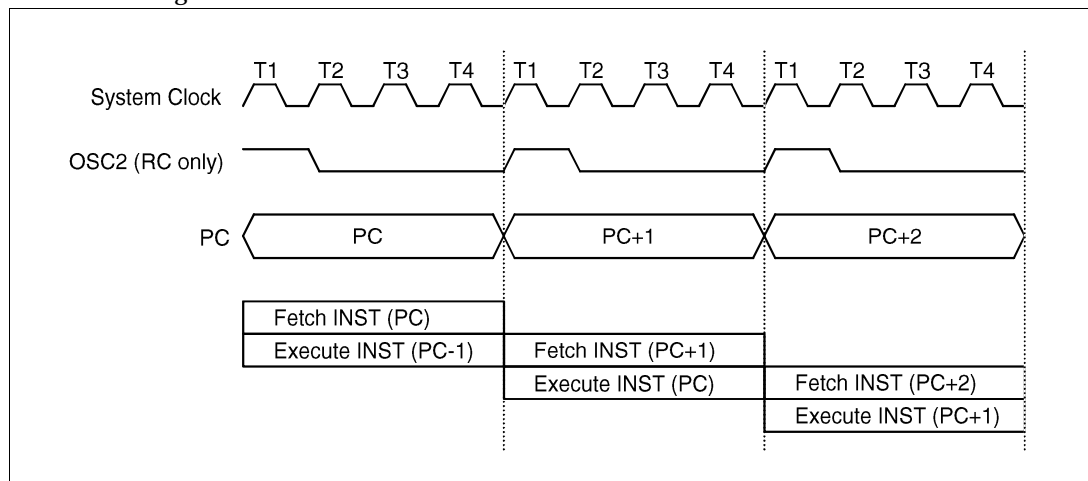
Execution Flow
