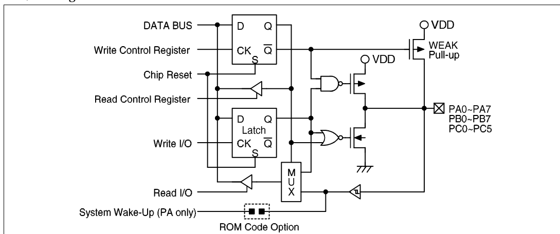
Input/Output Ports
