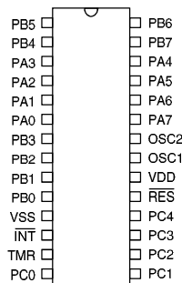
28SDIP-A-0
