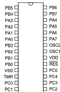
28SDIP-C-0
