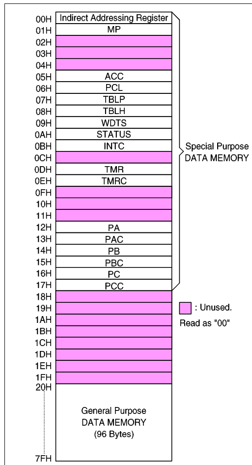
RAM Mapping
