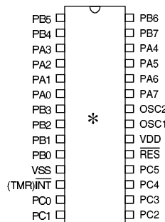
28SDIP-B-0
