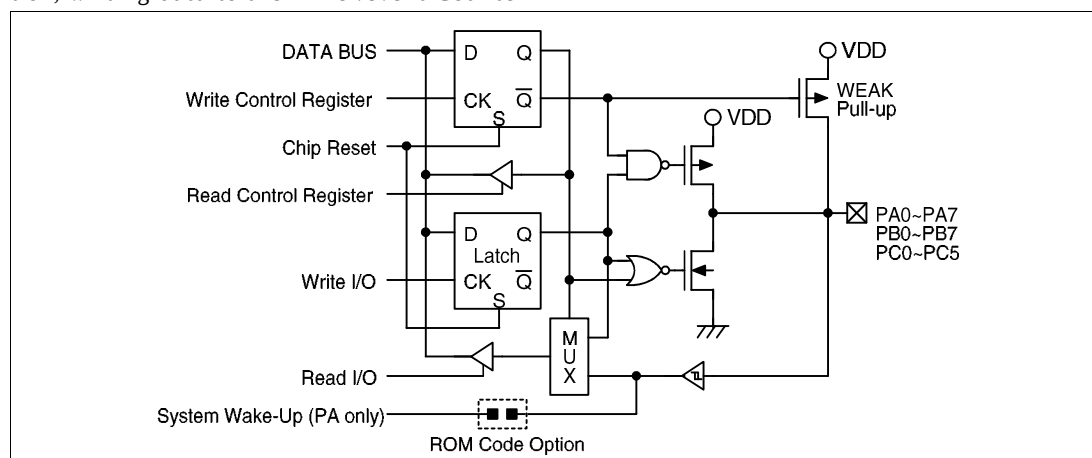
Input/Output Ports
