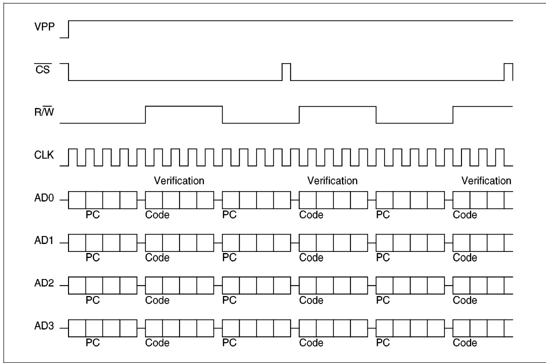
Non-successive Verification
