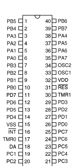
HT48C75 – 40 DIP-B-0
