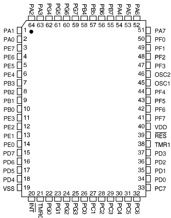
HT48C75 - 64 QFP-A-0
