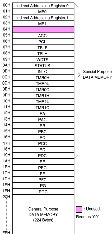
RAM mapping
