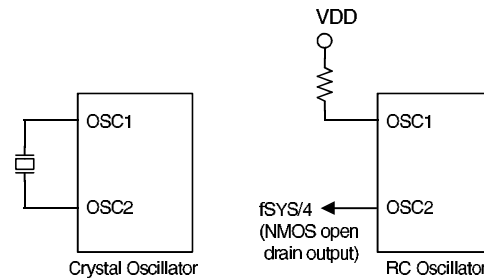
System oscillator
