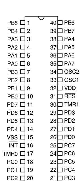
HT48C75 - 40 DIP-A-0
