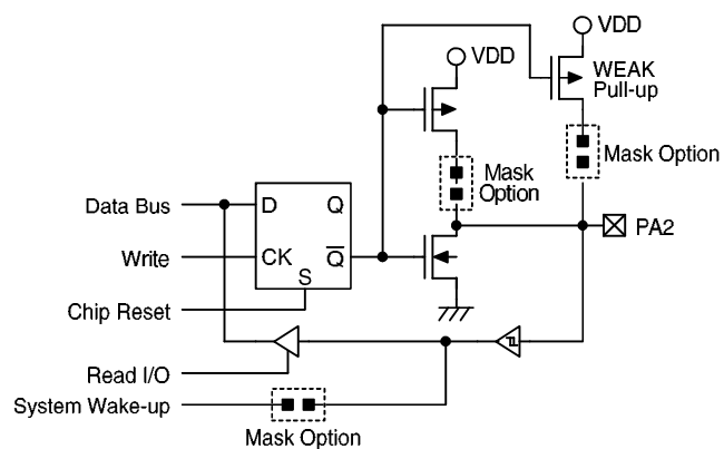
PA2 input/output line
