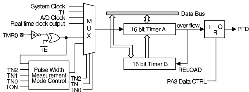
Timer/event counter
