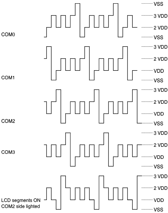
LCD driver output (1/4 duty, 1/3 bias)
