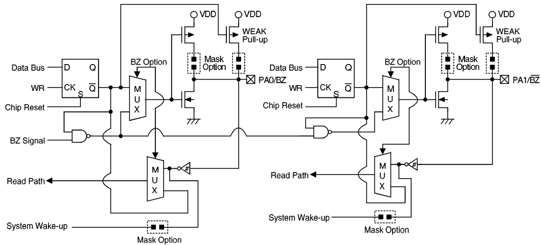
PA0/BZ, PA1/ \overline{\text{BZ}} input/output lines
