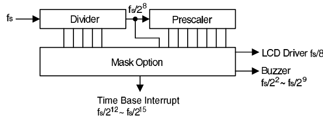
Time base
