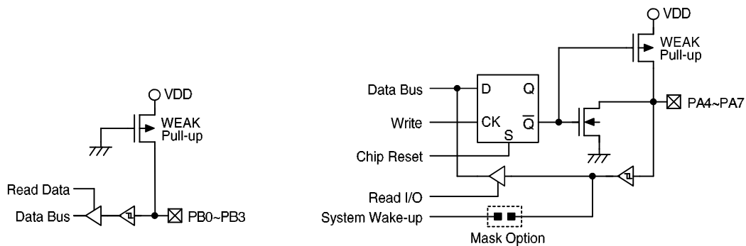
PA4~PA7 input/output lines
