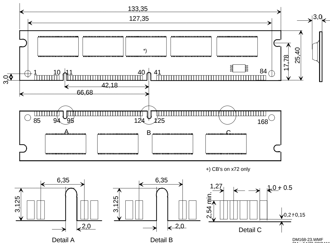
L-DIM-168-23 SDRAM DIMM Module package
