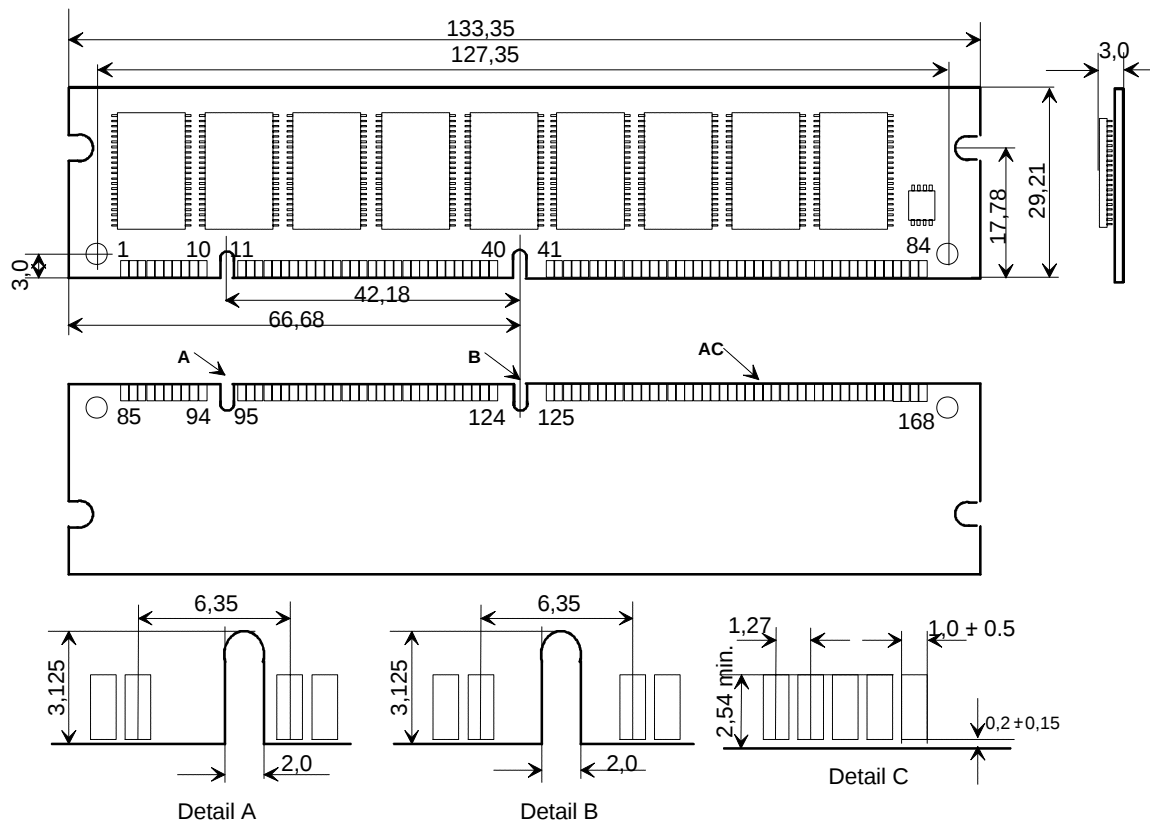
L-DIM-168-27 SDRAM DIMM Module package
