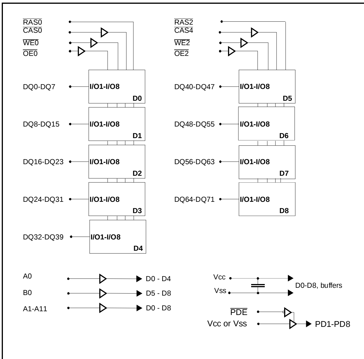
Block Diagram
