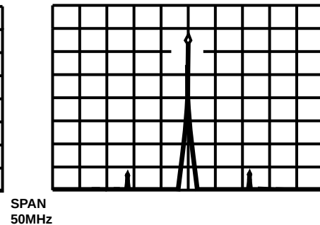
OUTPUT WITH EMITTER DEGENERATION R_{EE} = 4.7\Omega
