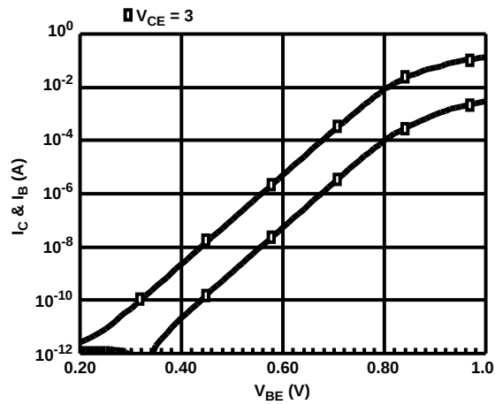
FIGURE 3. GUMMEL PLOT
