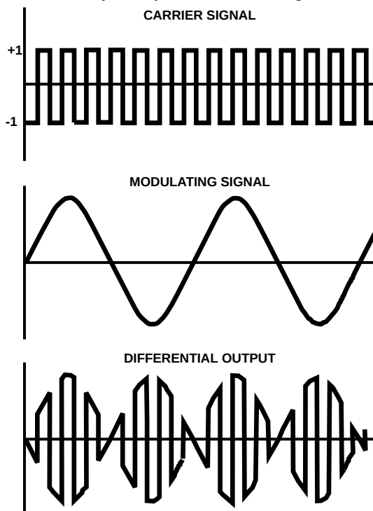
FIGURE 6. TYPICAL MODULATOR SIGNALS
