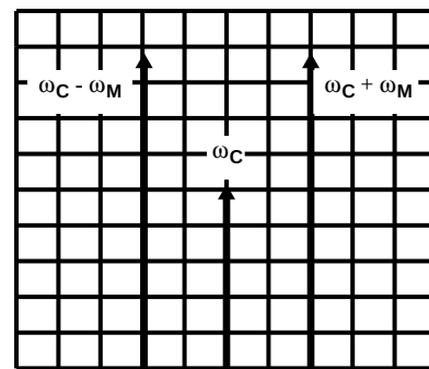
FIGURE 7A. UP CONVERSION OR SUPPRESSED CARRIER AM
