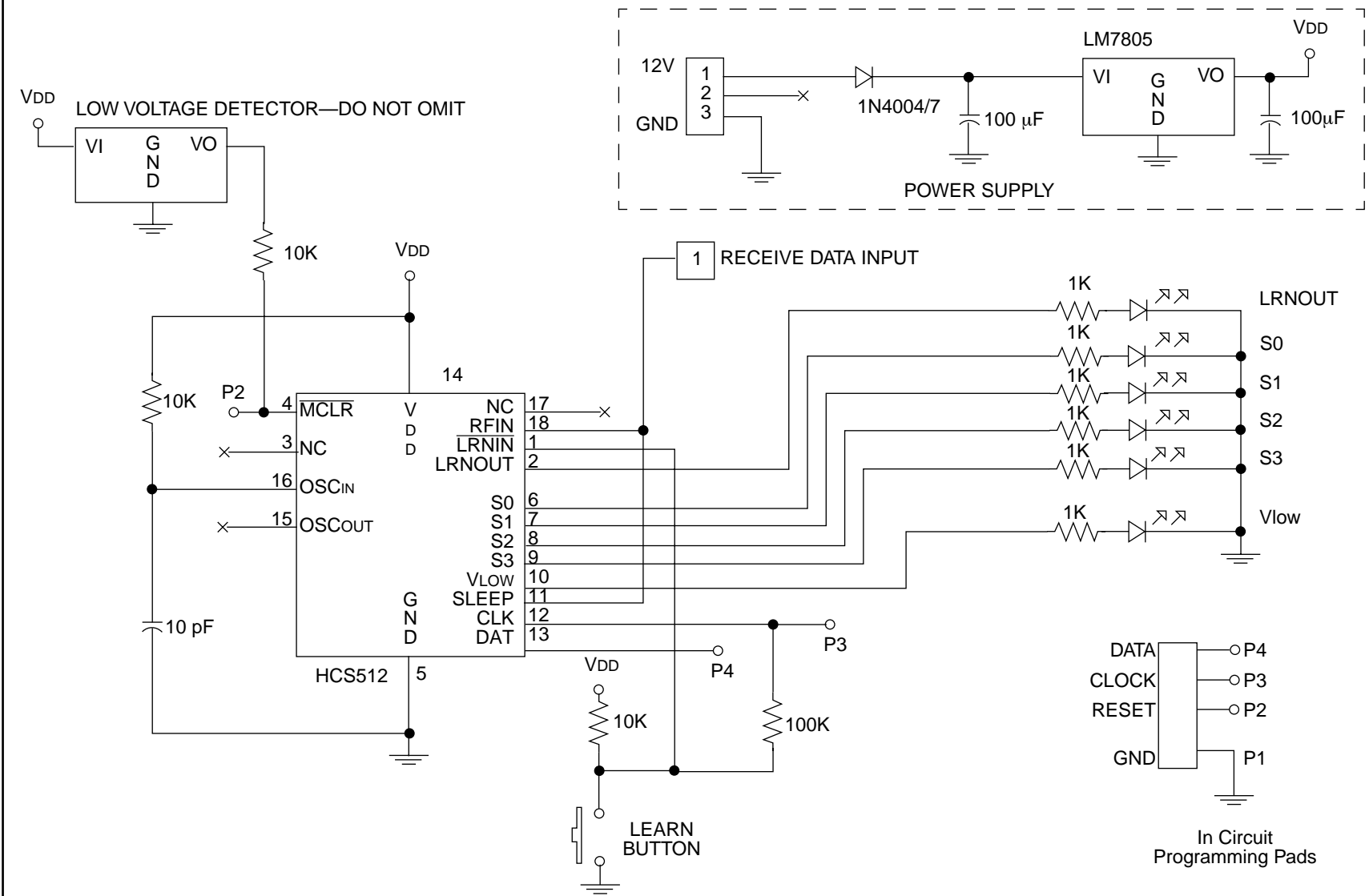
FIGURE 9-3: TYPICAL DECODER APPLICATION CIRCUIT
