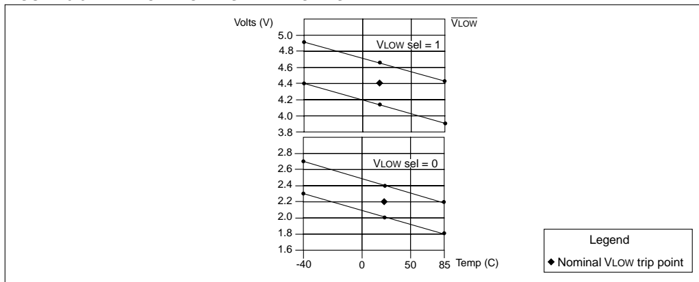
FIGURE 5-3: TYPICAL VOLTAGE TRIP POINTS
