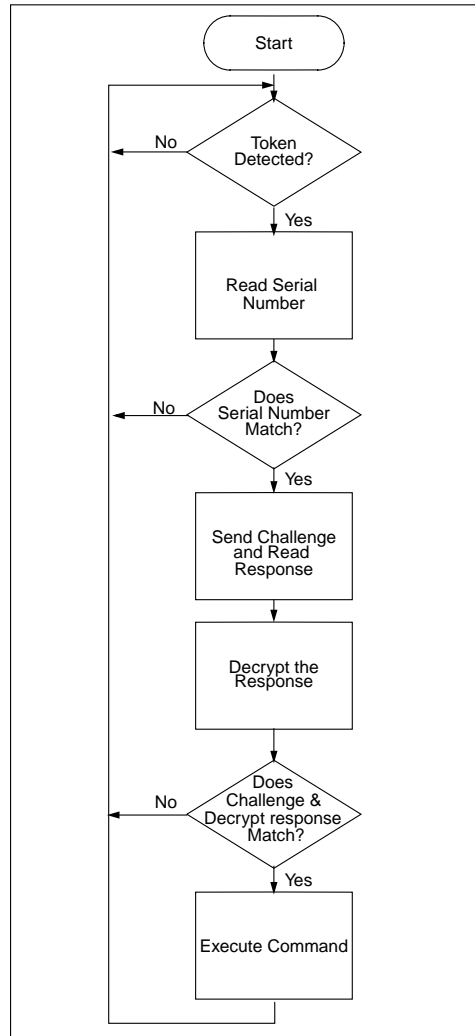
FIGURE 4-8: BASIC OPERATION OF AN IFF RECEIVER (DECODER)
