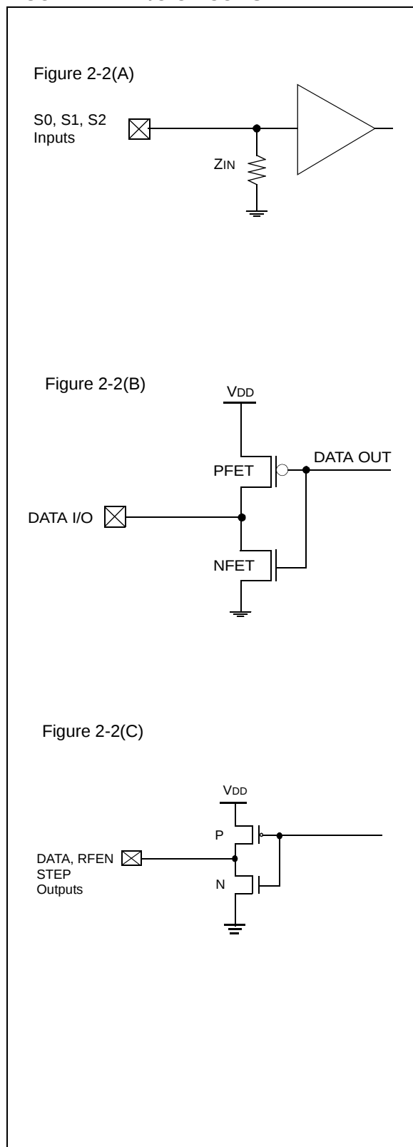
FIGURE 2-2: I/O CIRCUITS
