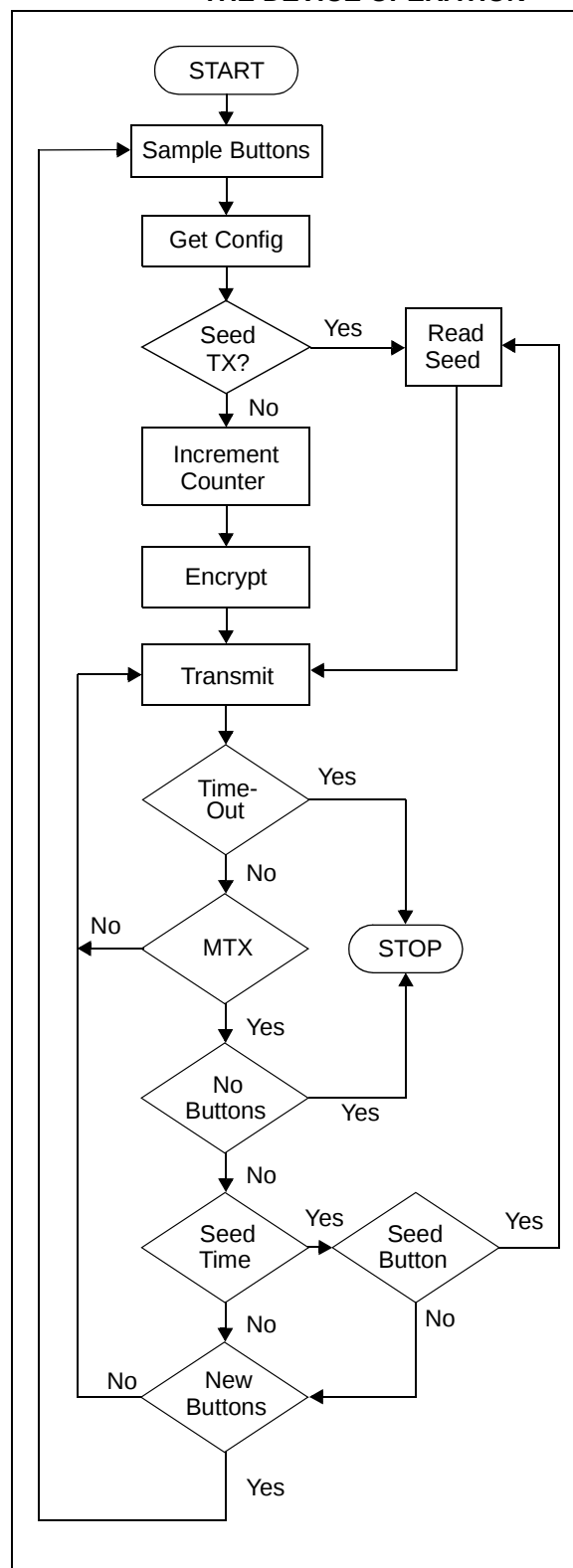
FIGURE 2-3: BASIC FLOW DIAGRAM OF THE DEVICE OPERATION
