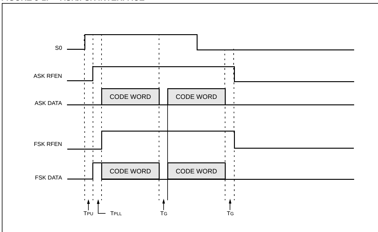
FIGURE 5-1: ASK/FSK INTERFACE
