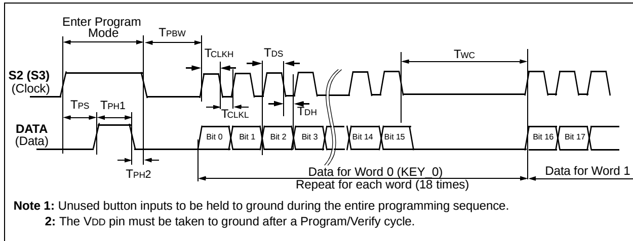
FIGURE 5-1: PROGRAMMING WAVEFORMS
