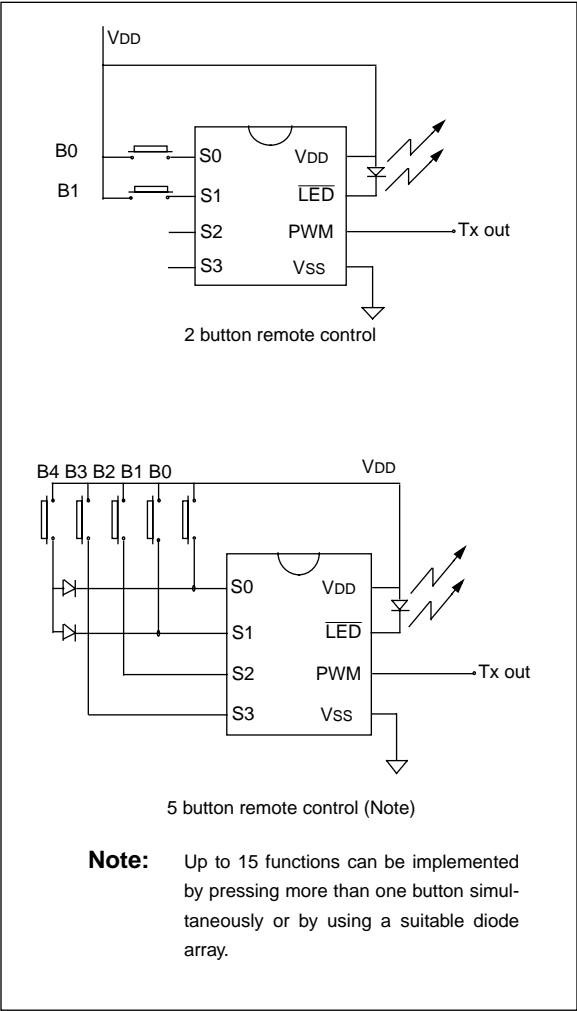
FIGURE 2-1: TYPICAL CIRCUITS
