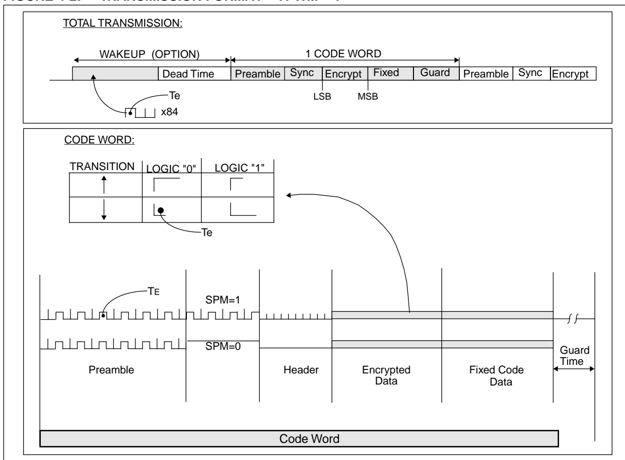
FIGURE 4-2: TRANSMISSION FORMAT—VPWM = 1
