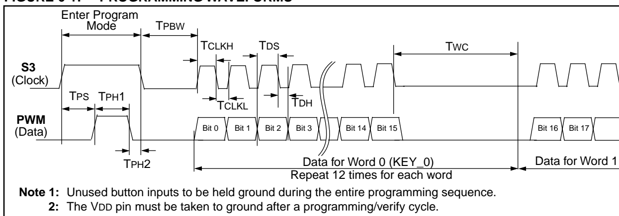
FIGURE 6-2: VERIFY WAVEFORMS
