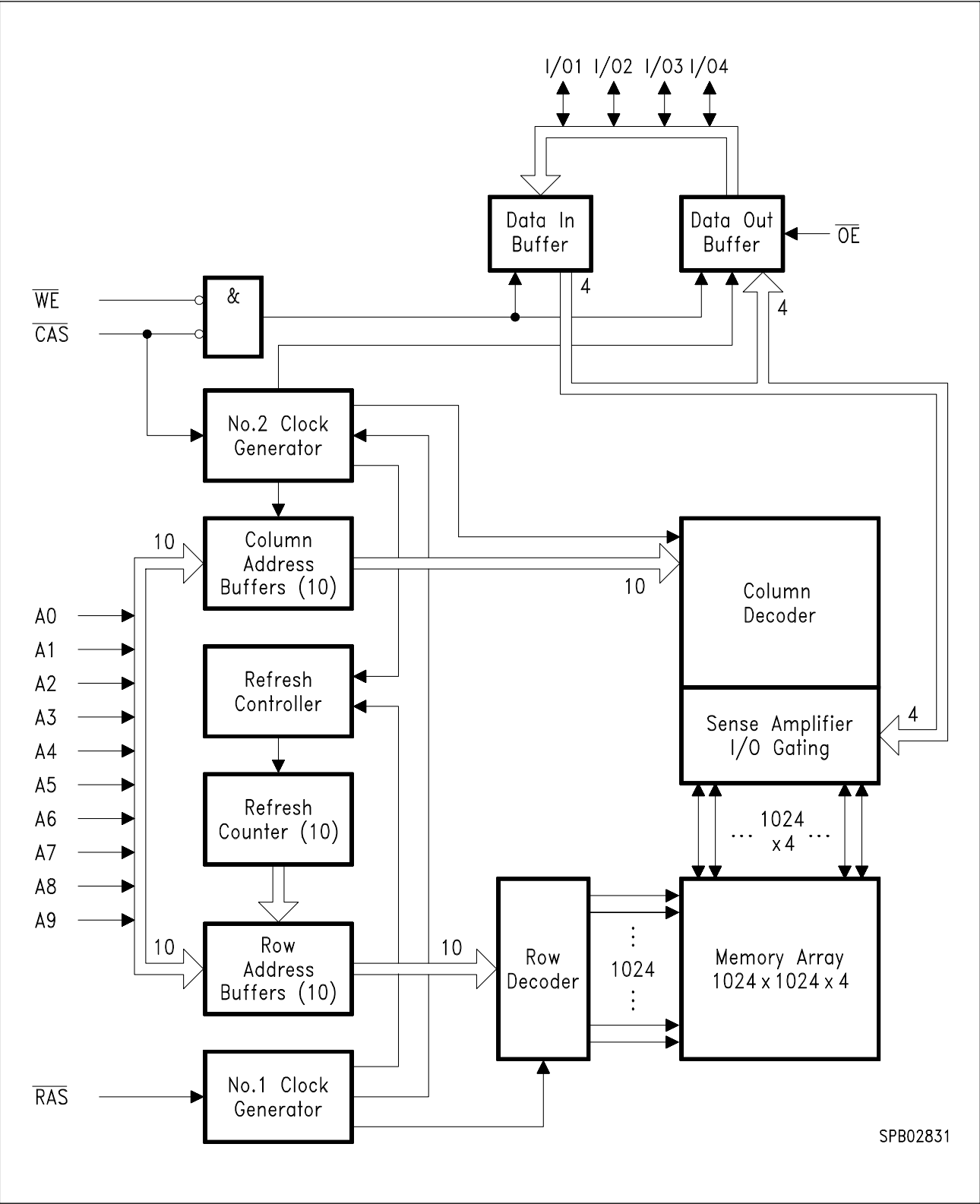
Block Diagram
