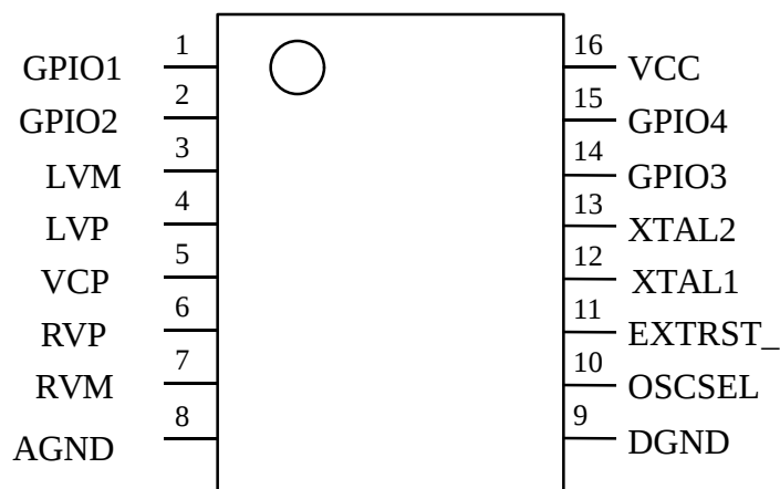
16-pin SOP
