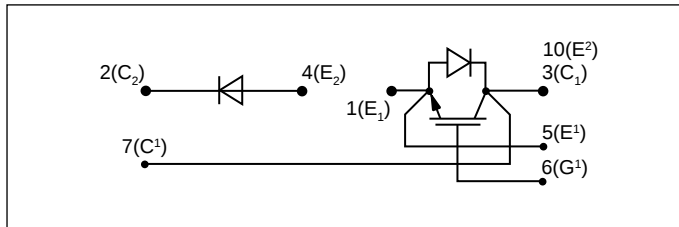
Fig.1 Chopper circuit diagram
