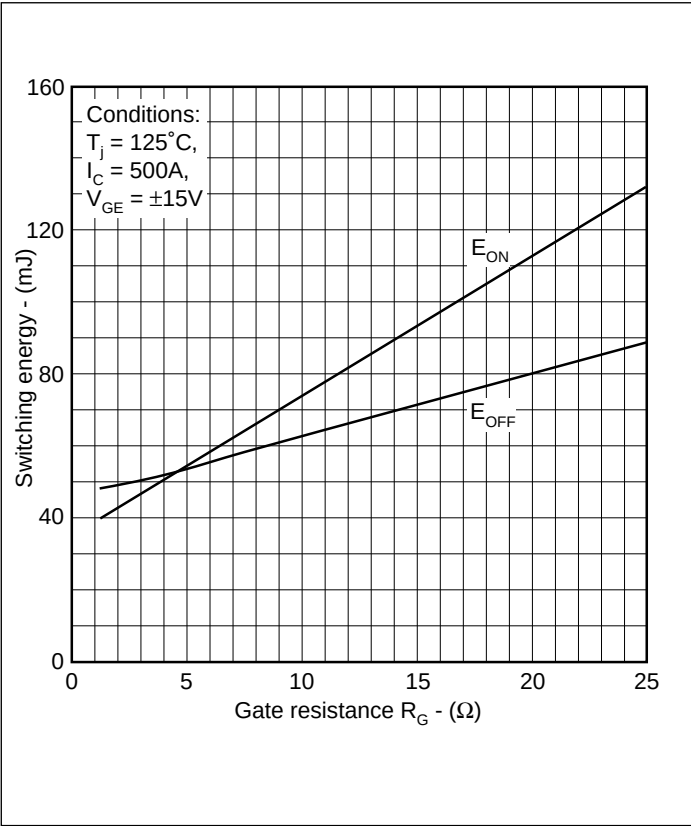
Fig.11 Typical switching energy @125°C
