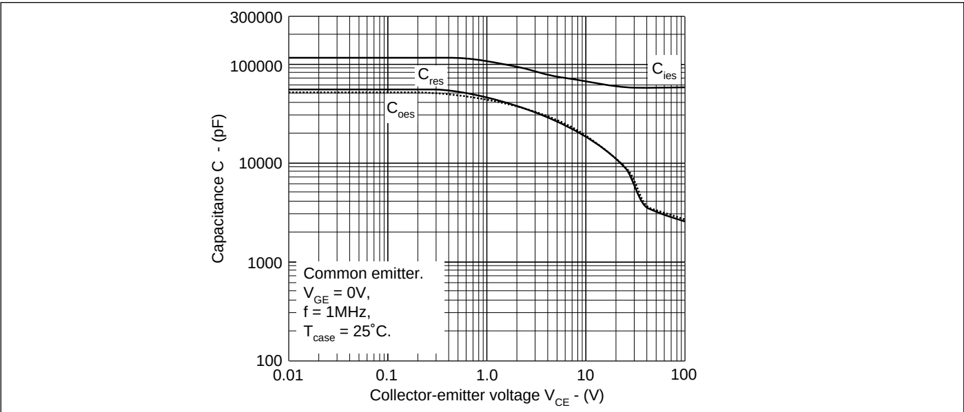
Fig.13 Typical capacitance
