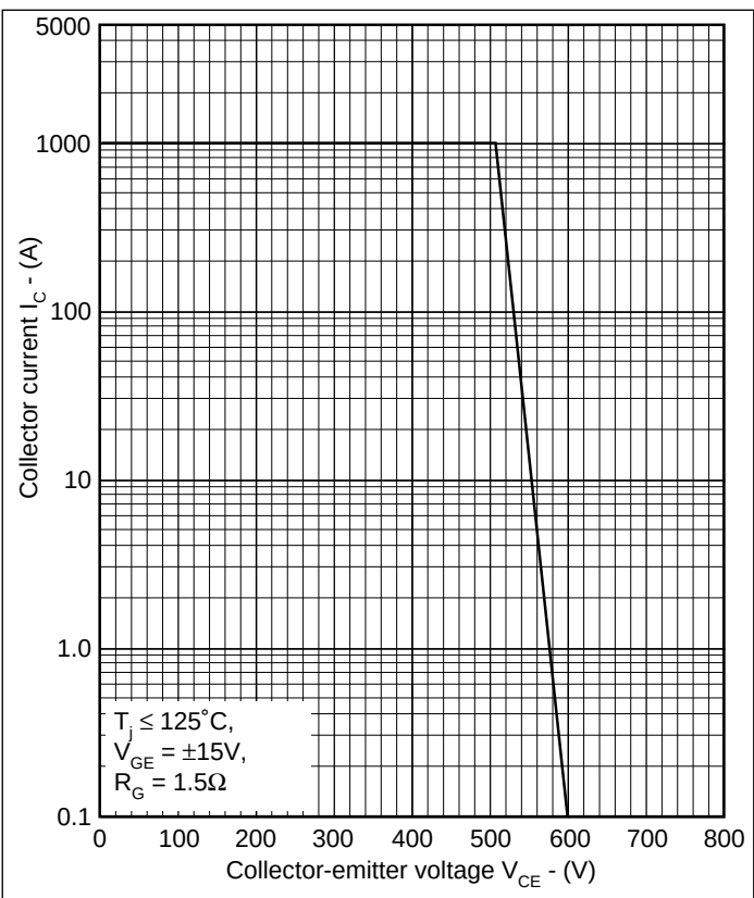
Fig.12 Reverse bias safe operating area
