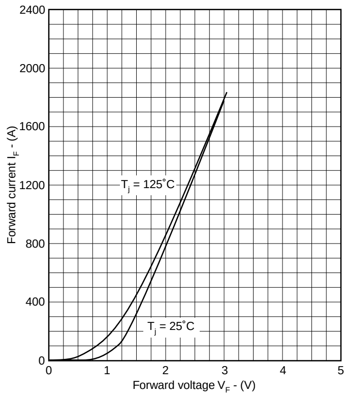
Fig.15 Typical diode forward characteristics
