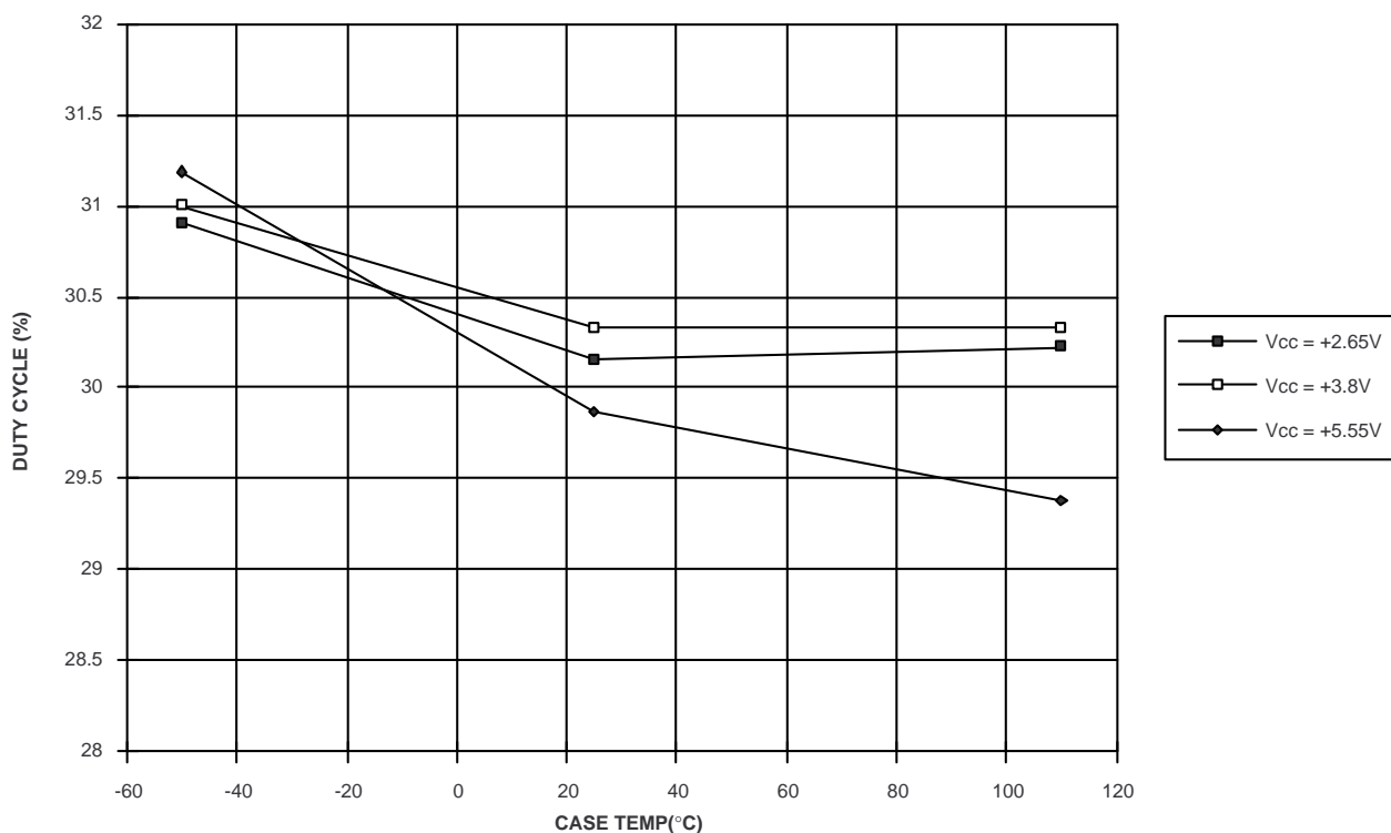
Fig. 25 Duty-cycle of MAG digital output (pin 12), sampled at 5.71MHz in a typical application circuit - RF I/P signal = 1575.42MHz CW, -85dBm - equivalent to 26dB excess noise from a typical GPS antenna
