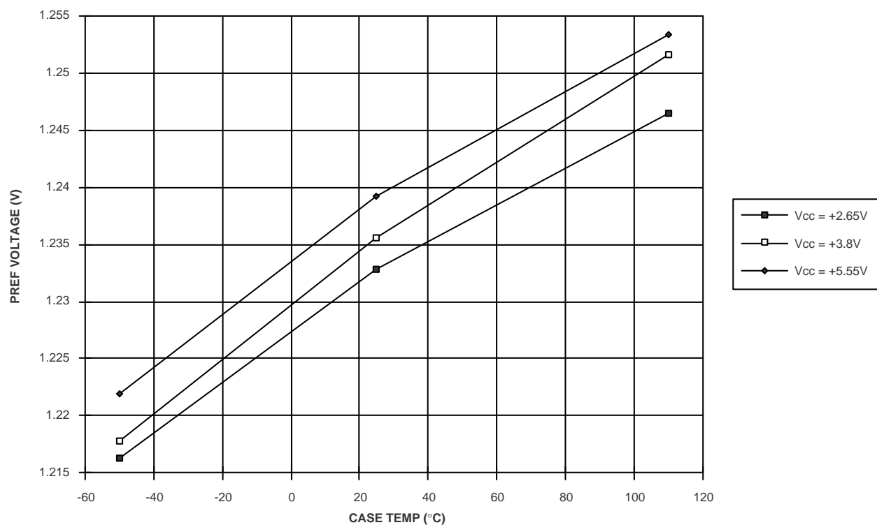
Fig. 24 Power-on Reset Threshold level
