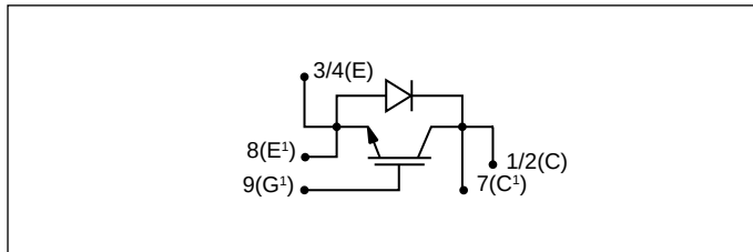
Fig.1 Single switch circuit diagram
