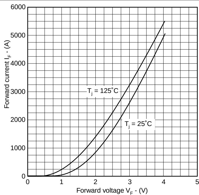
Fig.15 Typical diode forward characteristics
