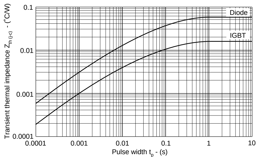
Fig.14 Transient thermal impedance
