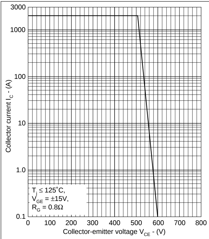
Fig.12 Reverse bias safe operating area
