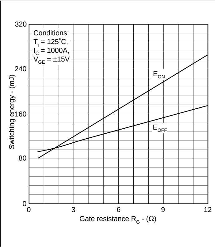
Fig.11 Typical switching energy @125°C
