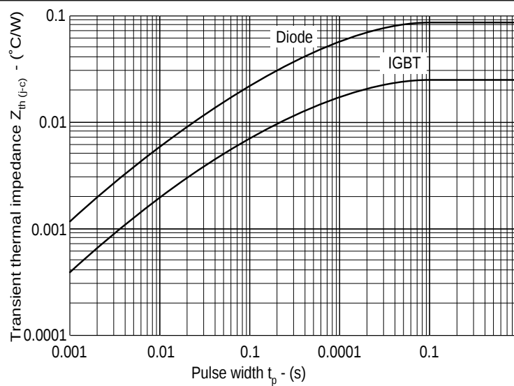
Fig.14 Transient thermal impedance
