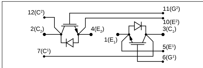
Fig.1 Half bridge circuit diagram
