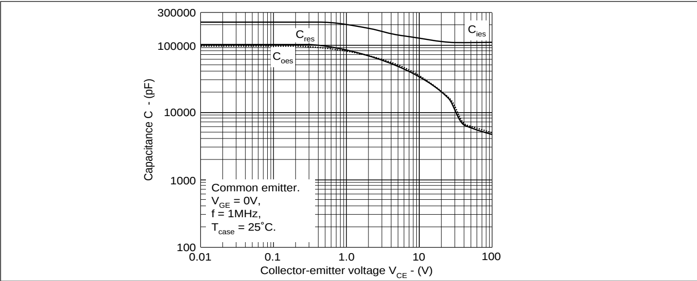
Fig.13 Typical capacitance
