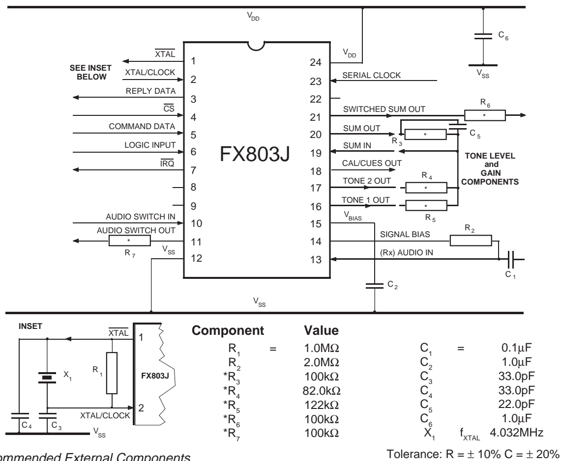
Fig.2 Recommended External Components
