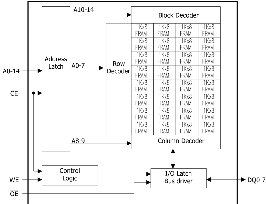
Figure 1. Block Diagram
