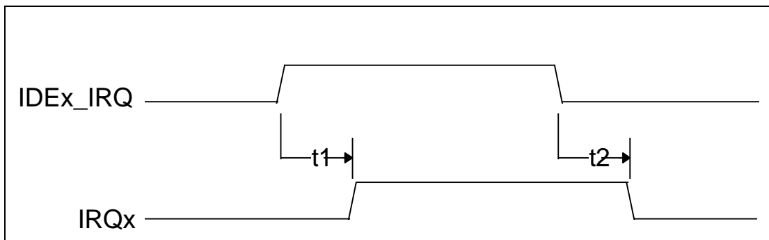
FIGURE 22 - IRQ TIMING
