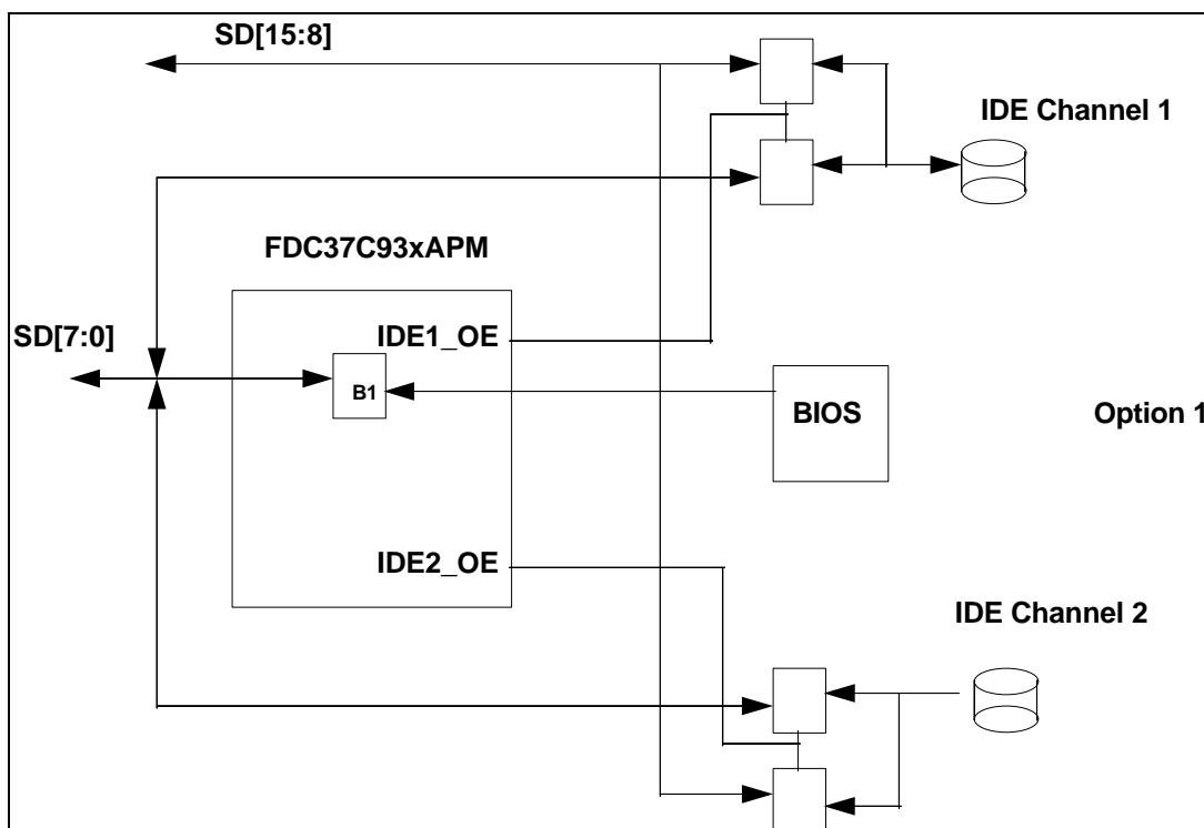
FIGURE 2 - IDE OUTPUT ENABLE OPTION 1I
