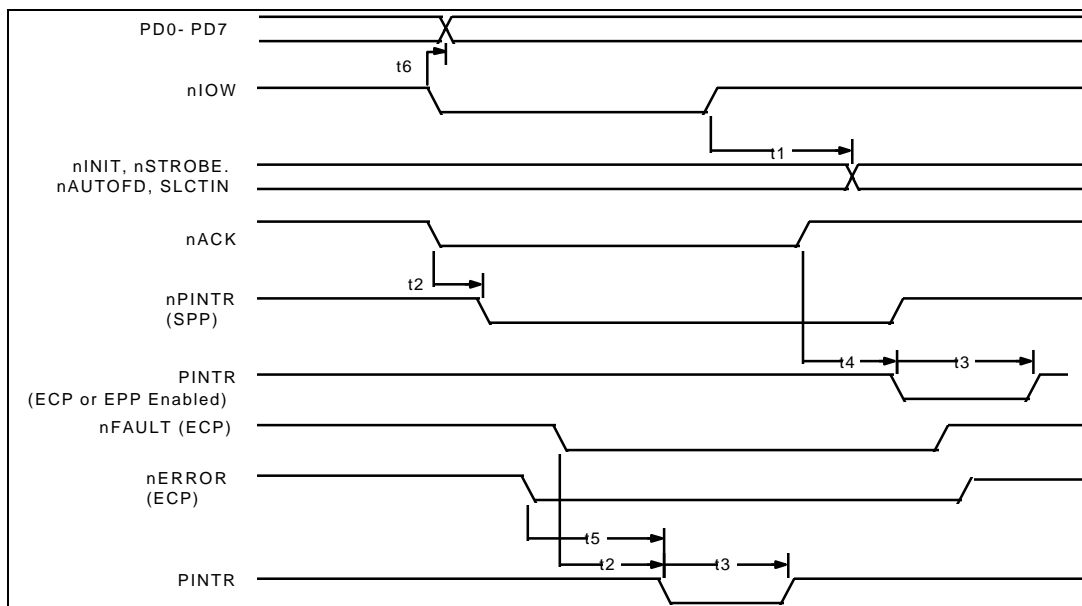
FIGURE 29 - PARALLEL PORT TIMING
