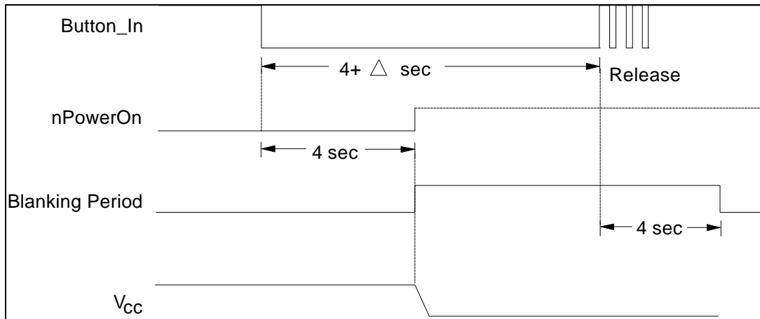
FIGURE 12 - BLANKING PERIOD
