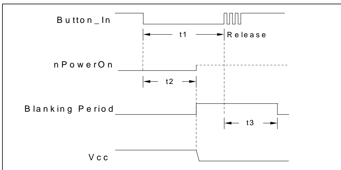
FIGURE 15B - BUTTON OVERRIDE TIMING
