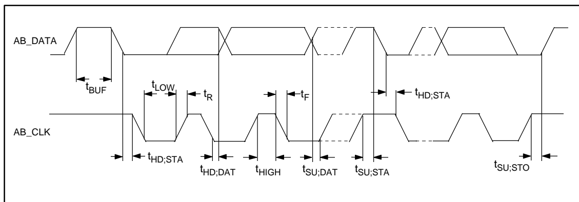
FIGURE 37 - ACCESS.BUS TIMING
