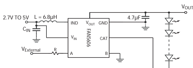
Analog Brightness Control
