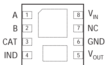
FAN5606 8-Lead 3x3mm MLP
