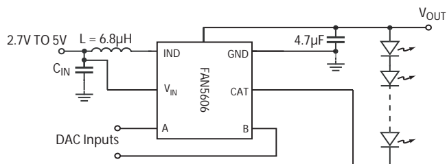
Digital Brightness Control
