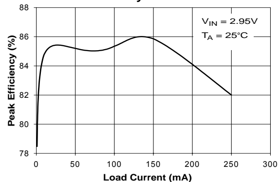
Peak Efficiency vs Load Current
