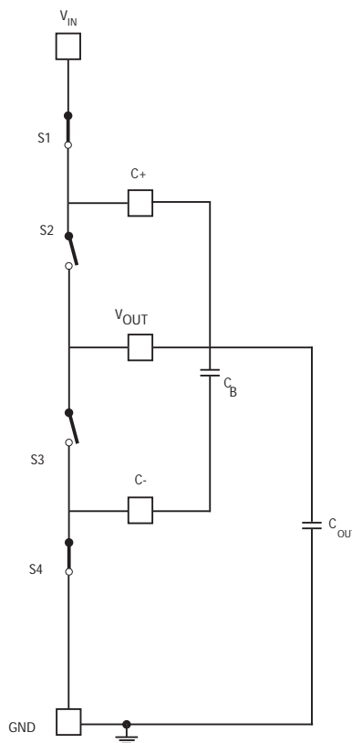
Figure. 1(B) 1:1 configuration Switch 3 is always off and Switch 4 is always on Switches 1 and 2 are in phase 1 Reverse the position of switches 1&2 for phase 2
