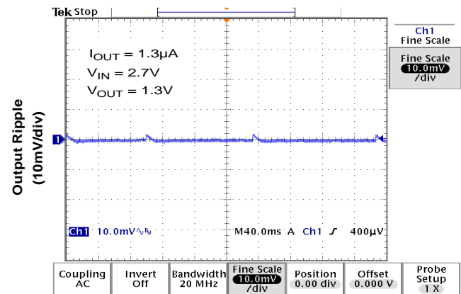
Output Ripple
