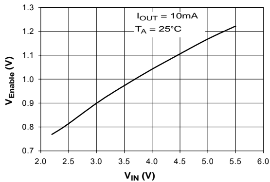
Enable Threshold vs Input Voltage
