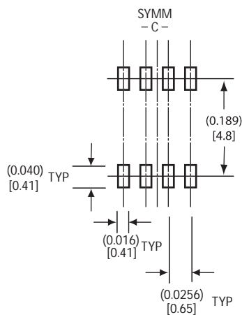
PCB LAND PATTERN
