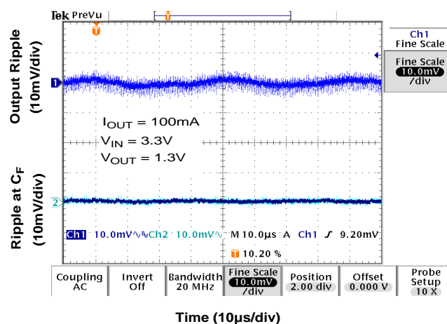
Figure 3. Effect of L-C Filter on output ripple
