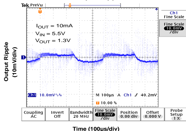
Output Ripple
