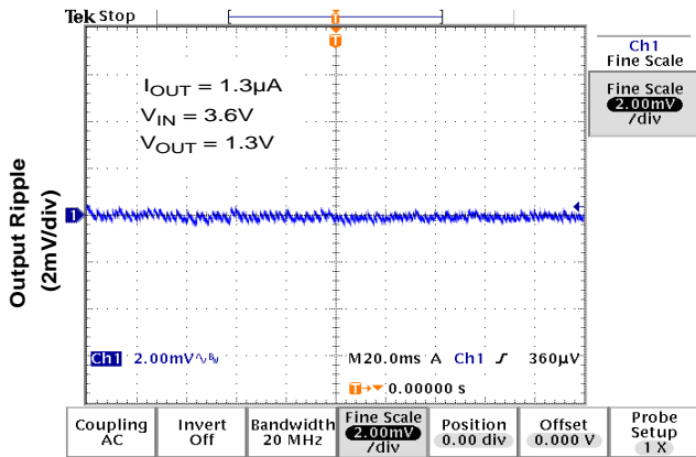
Output Ripple
