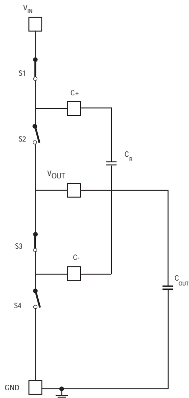
Figure. 1(A) 2:1 configuration Switches in charging phase Reverse all switches for pumping phase
