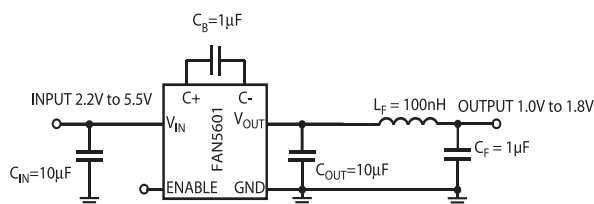
Figure 2. Optional L-C Filter
