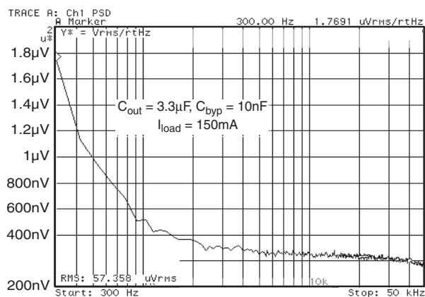
Noise Plot
