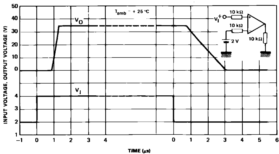
Figure 13 : Response Time.
