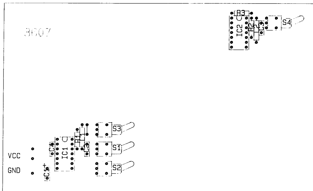
Figure 14. The layout and components placement of the demo-board
