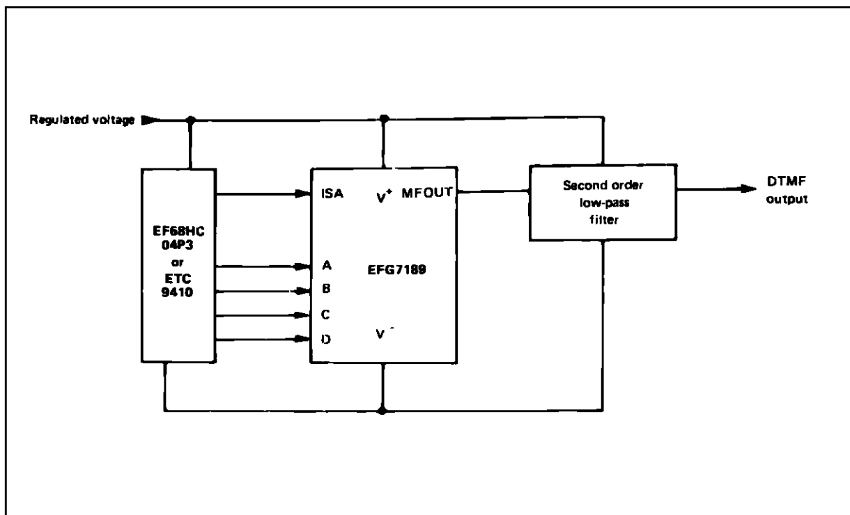
Figure 8 : Parallel Connection.
