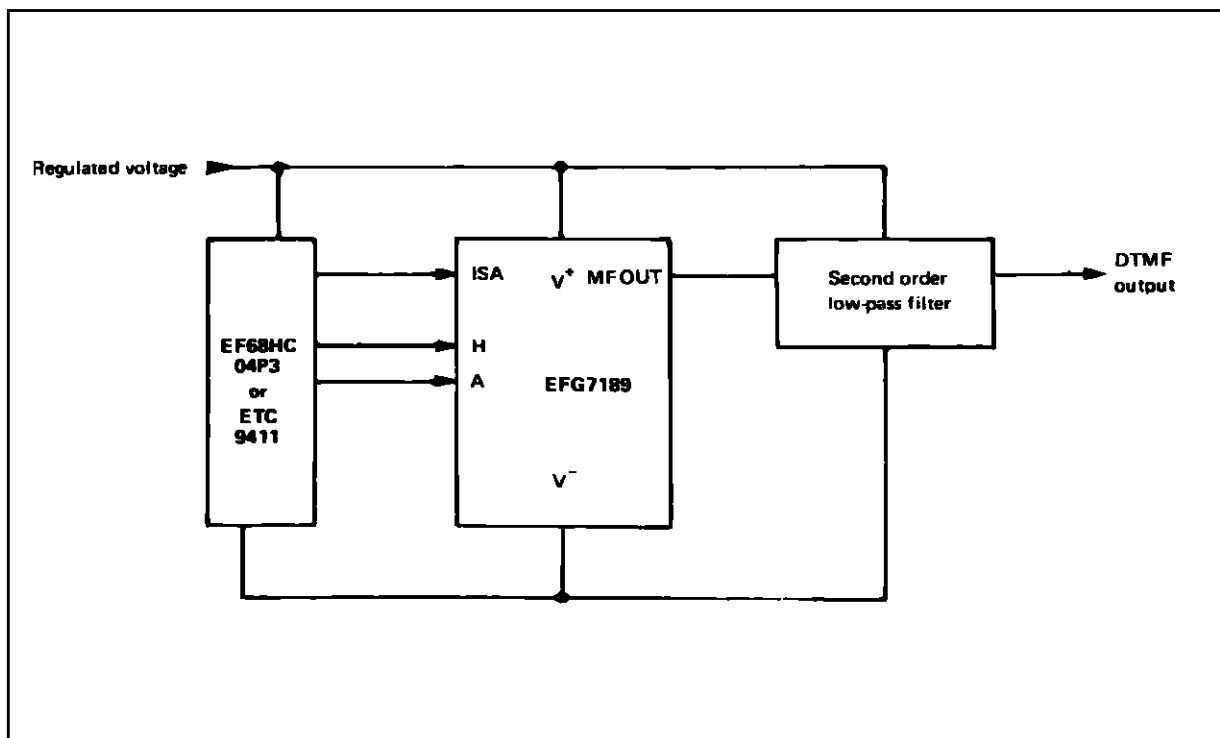
Figure 9 : Serial Connection.
