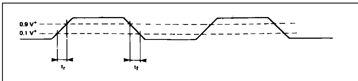
Figure 6 : Parallel Operating Mode (H = "1").
