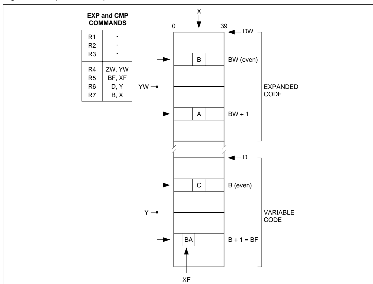
Figure 17 : Expansion/Compression Move
