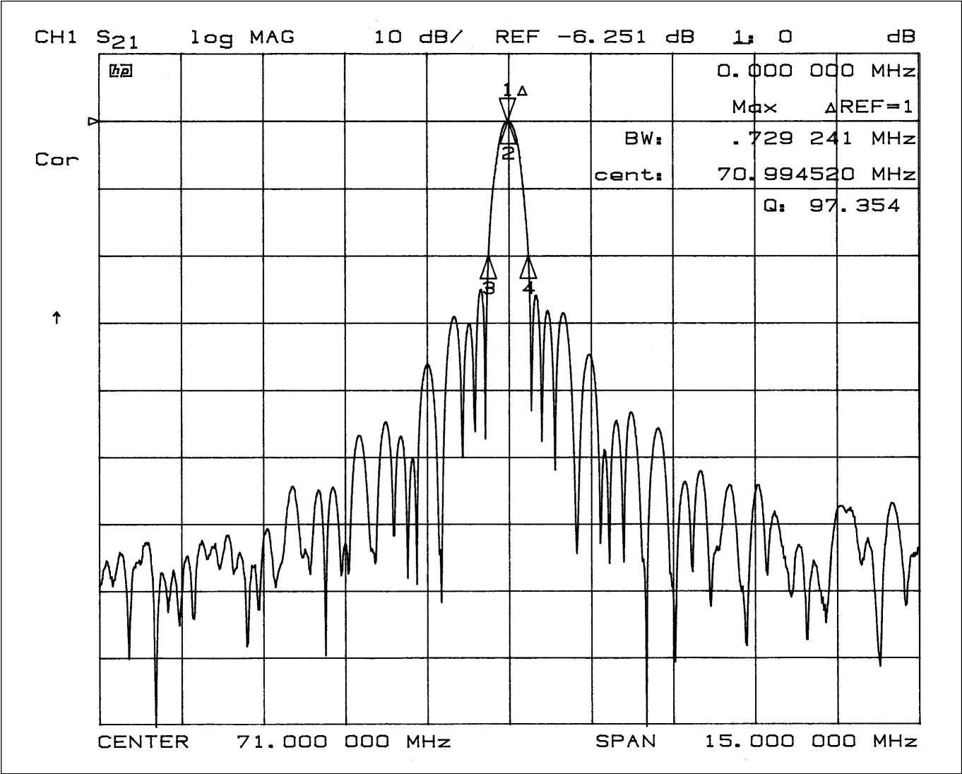
Figure 1: Amplitude Characteristics
