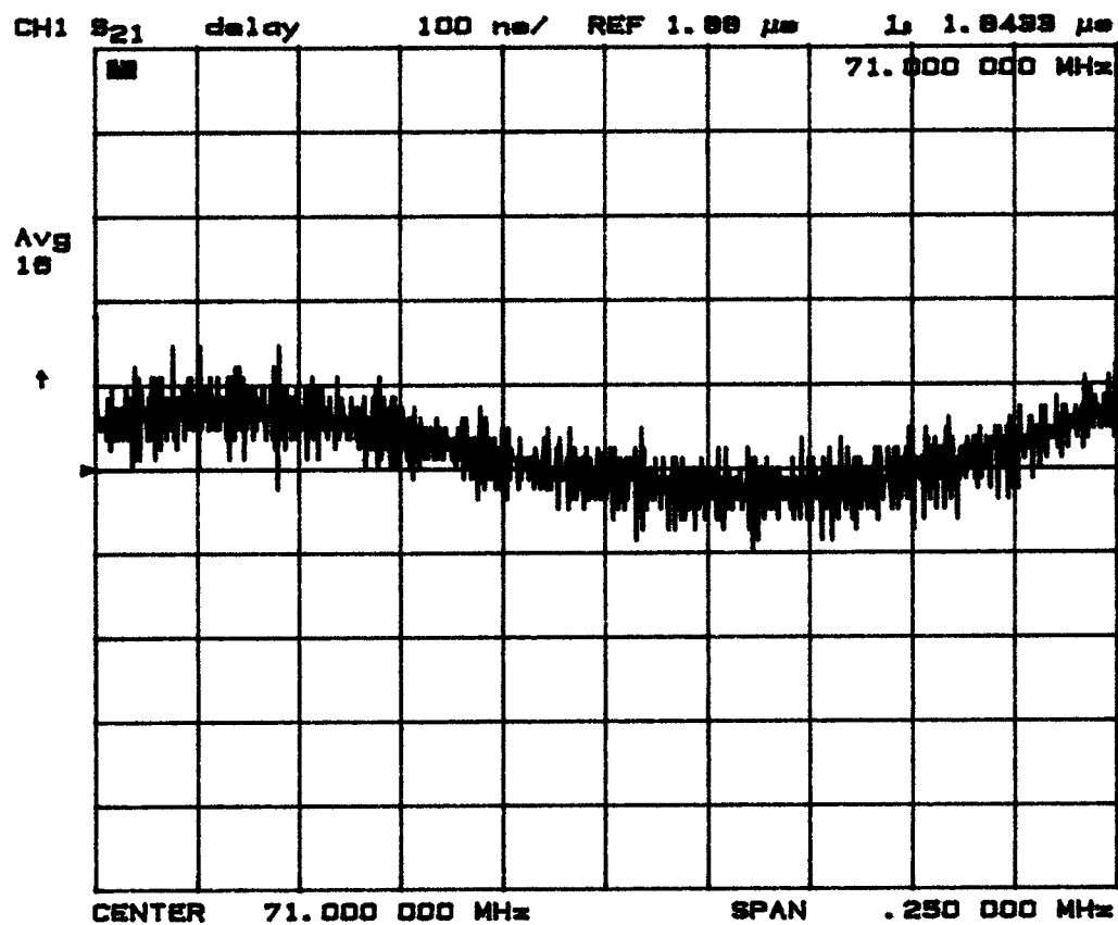
Figure 2: Group Delay Ripple Characteristics
