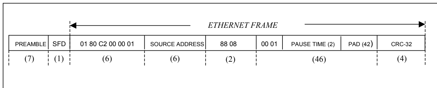
Figure 3. Pause-Control Frame
