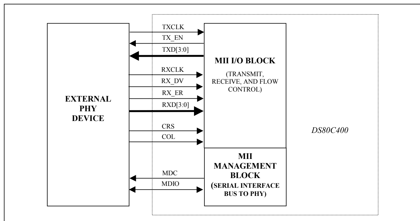
Figure 4. MII Block Diagram
