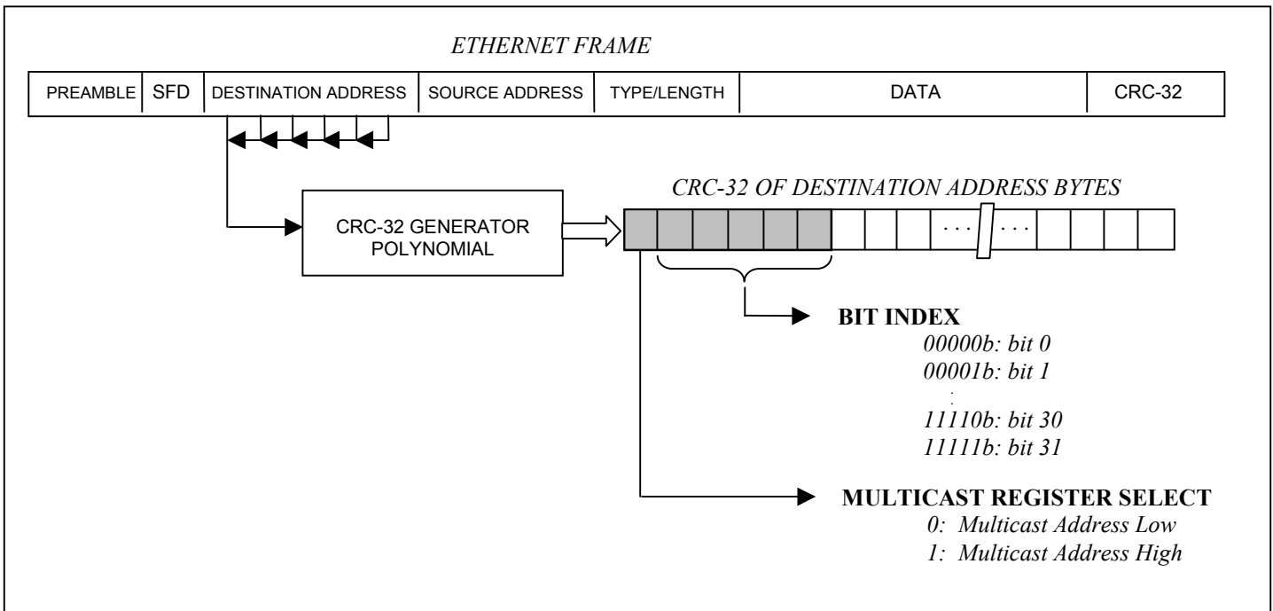
Figure 8. Hash Table Index Generation
