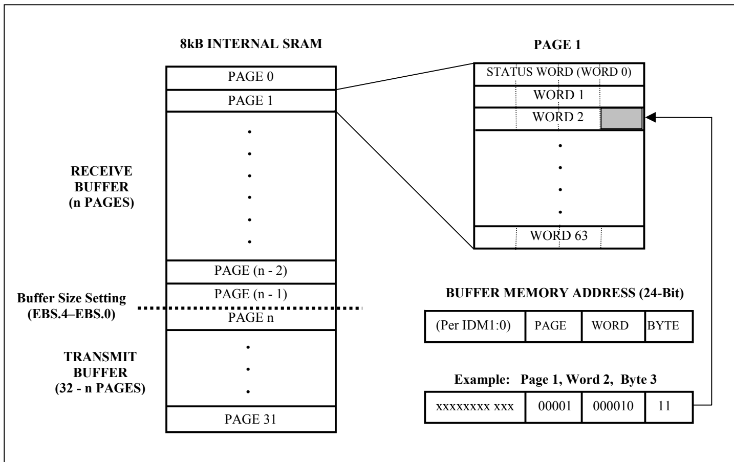
Figure 10. Transmit/Receive Data Buffer Memory
