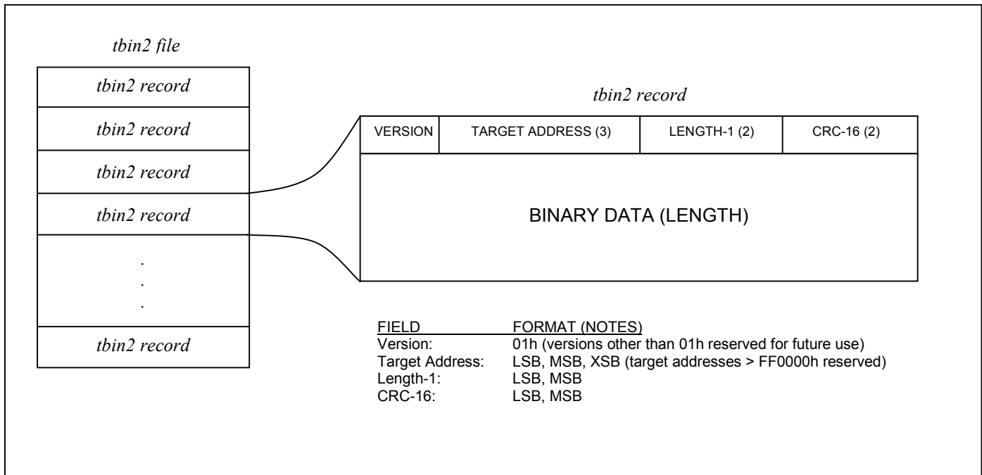
Figure 16. Dallas tbin2 Record and File Format
