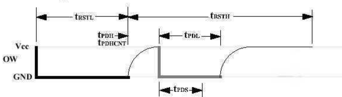
Initialization Sequence
