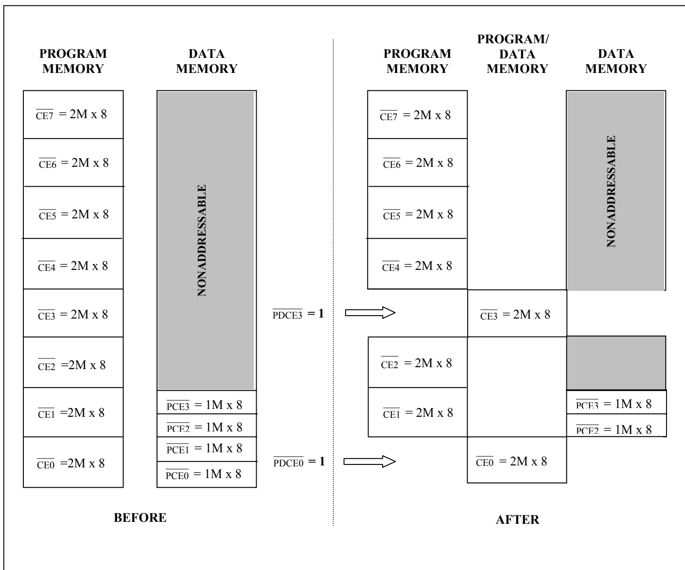
Figure 1. Example External Memory Map—Merged Program/Data
