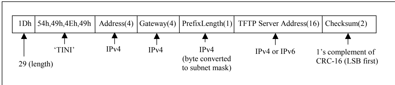
Figure 15. 1-Wire IP and TFTP Server IP Address Format
