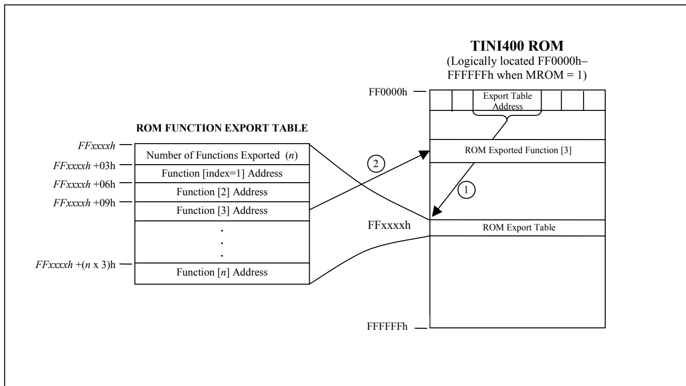
Figure 18. Finding the Location of an Exported ROM Function
