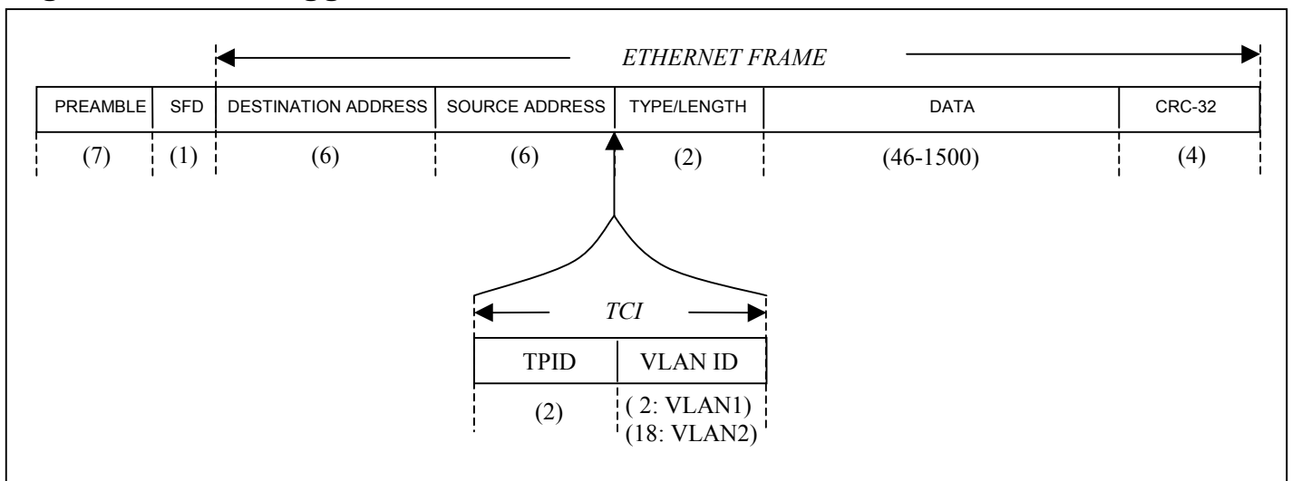
Figure 9. VLAN Tagged Frame
