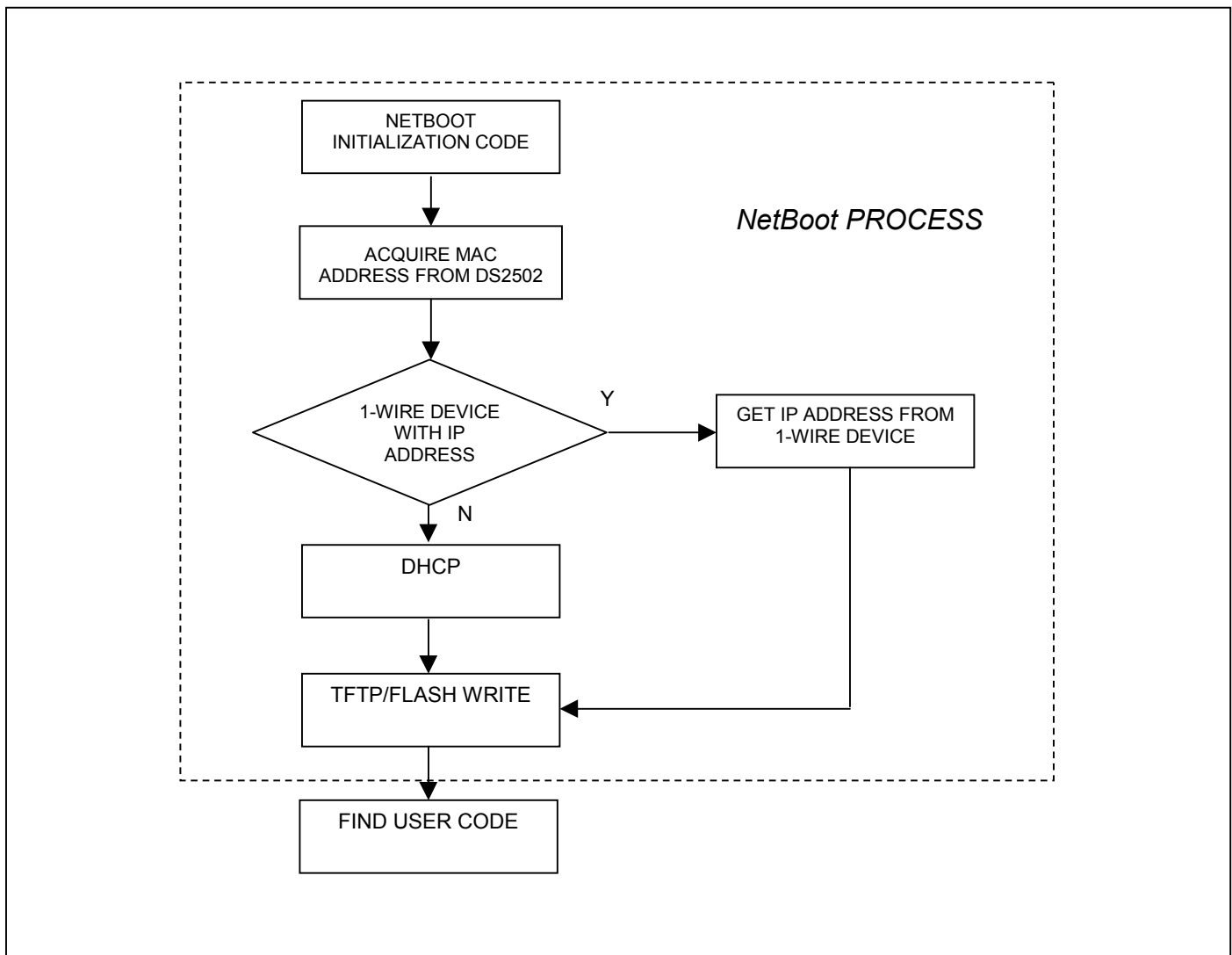
Figure 14. NetBoot Code Flow Chart
