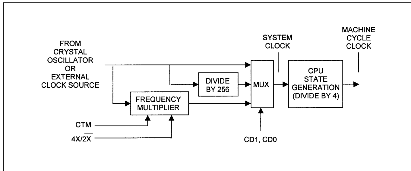
Figure 20. System Clock Control Diagram
