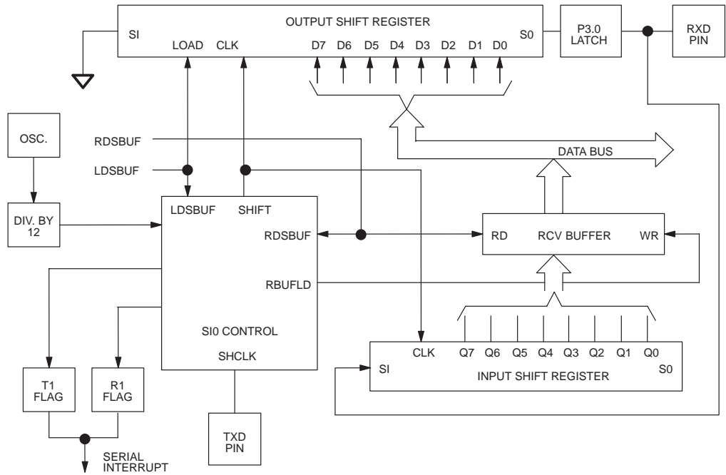
MODE 0 BLOCK DIAGRAM AND TIMING Figure 14-2
