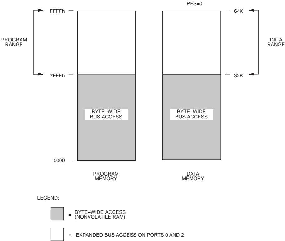
NON-PARTITIONABLE MEMORY MAP FOR DS5001, DS5002 SERIES Figure 4-6
