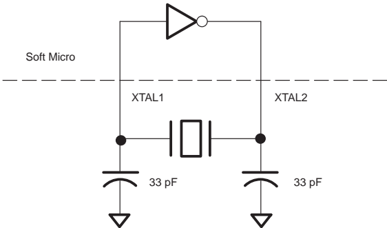
CRYSTAL CONNECTION Figure 15-1
