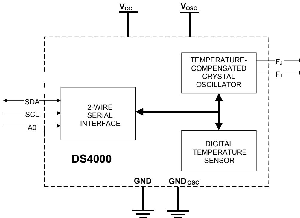
Figure 1. BLOCK DIAGRAM
