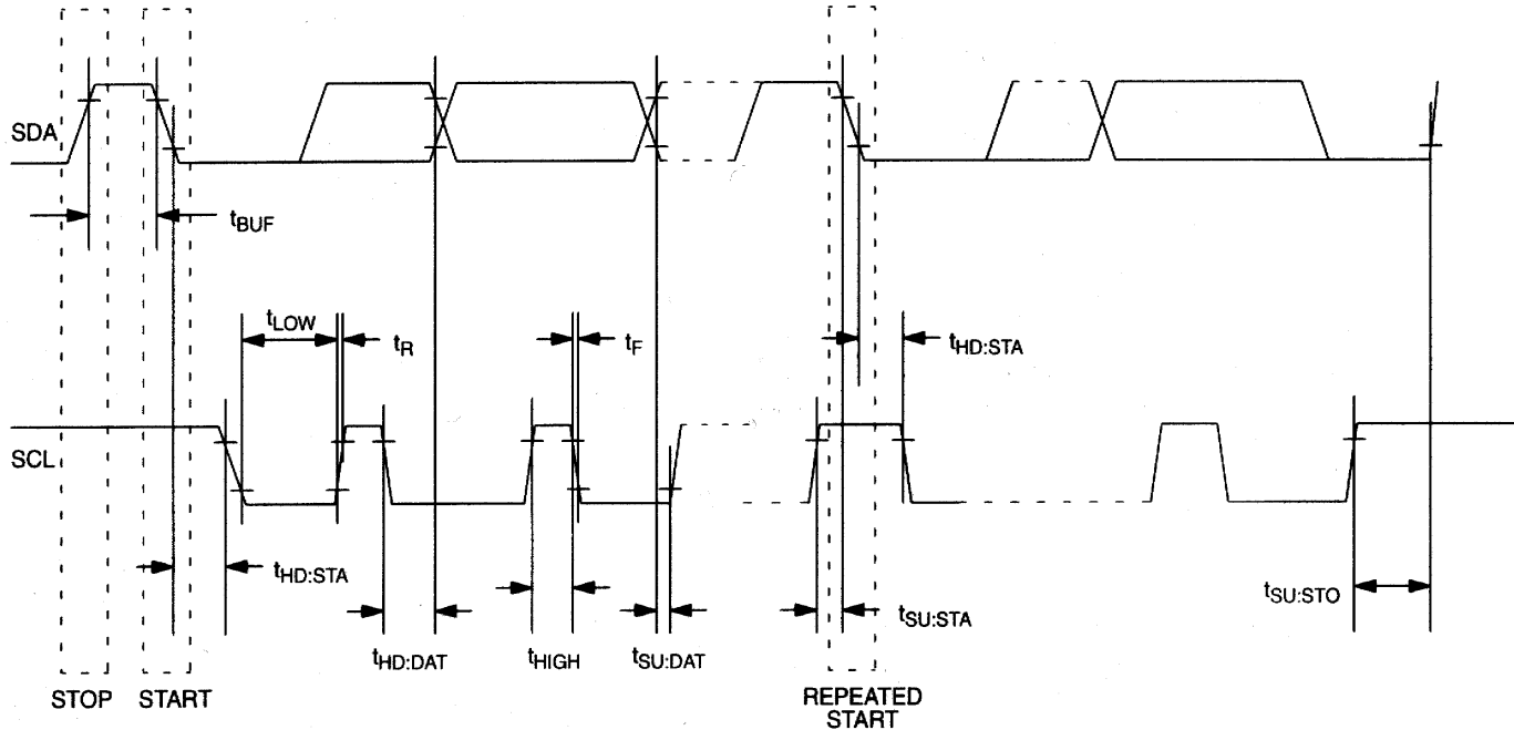
Figure 4. TIMING DIAGRAM
