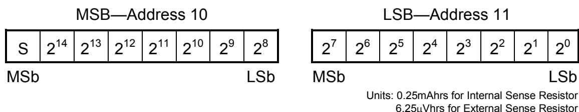
Figure 5. CURRENT ACCUMULATOR FORMAT
