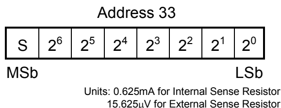
Figure 6. CURRENT OFFSET BIAS
