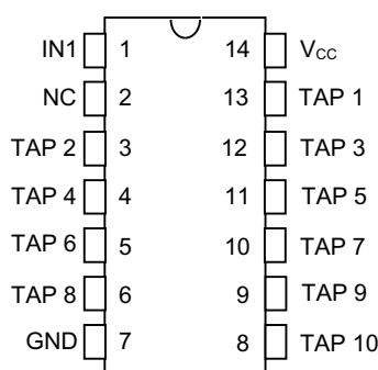
DS1010 14-Pin DIP (300-mil) See Mech. Drawings Section
