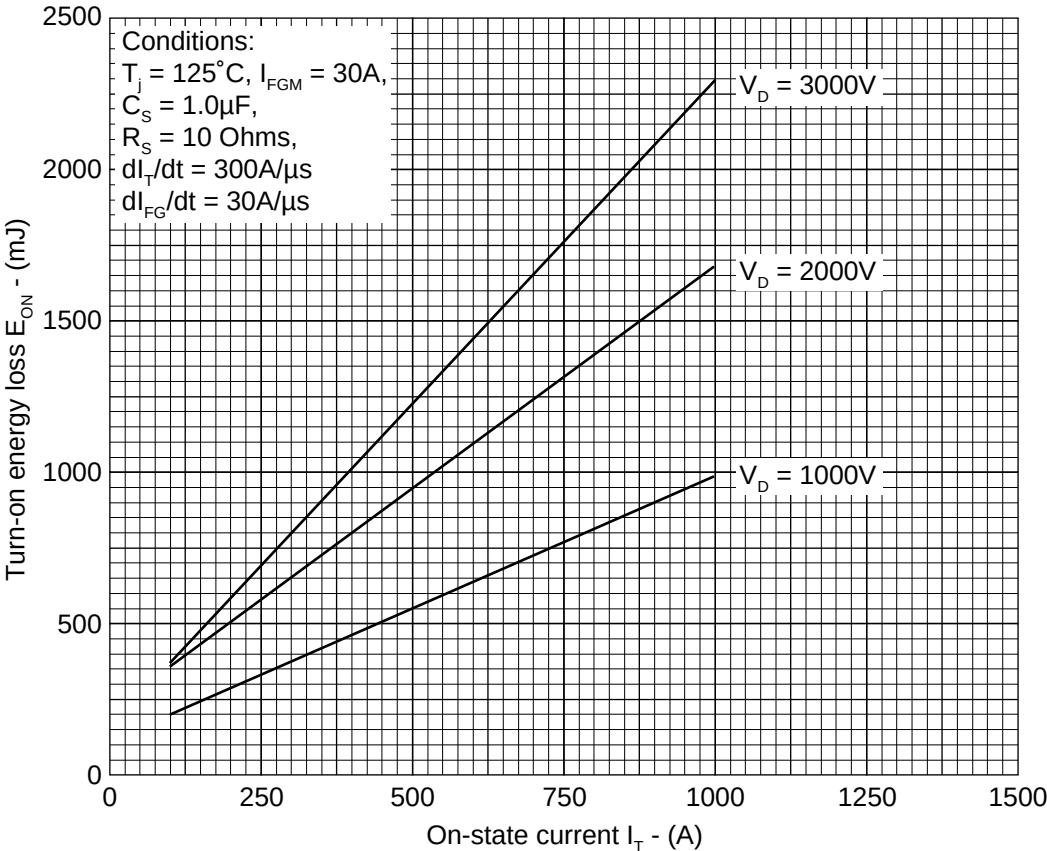
FIG. 10 TURN-ON ENERGY vs ON-STATE CURRENT
