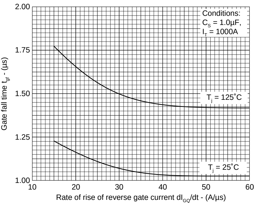
FIG. 23 GATE FALL TIME vs RATE OF RISE OF REVERSE GATE CURRENT
