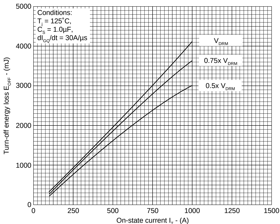
FIG. 17 TURN-OFF ENERGY vs ON-STATE CURRENT
