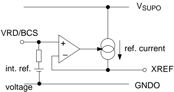
Fig. 4-16: Input pins XREF and VRD/BCS
