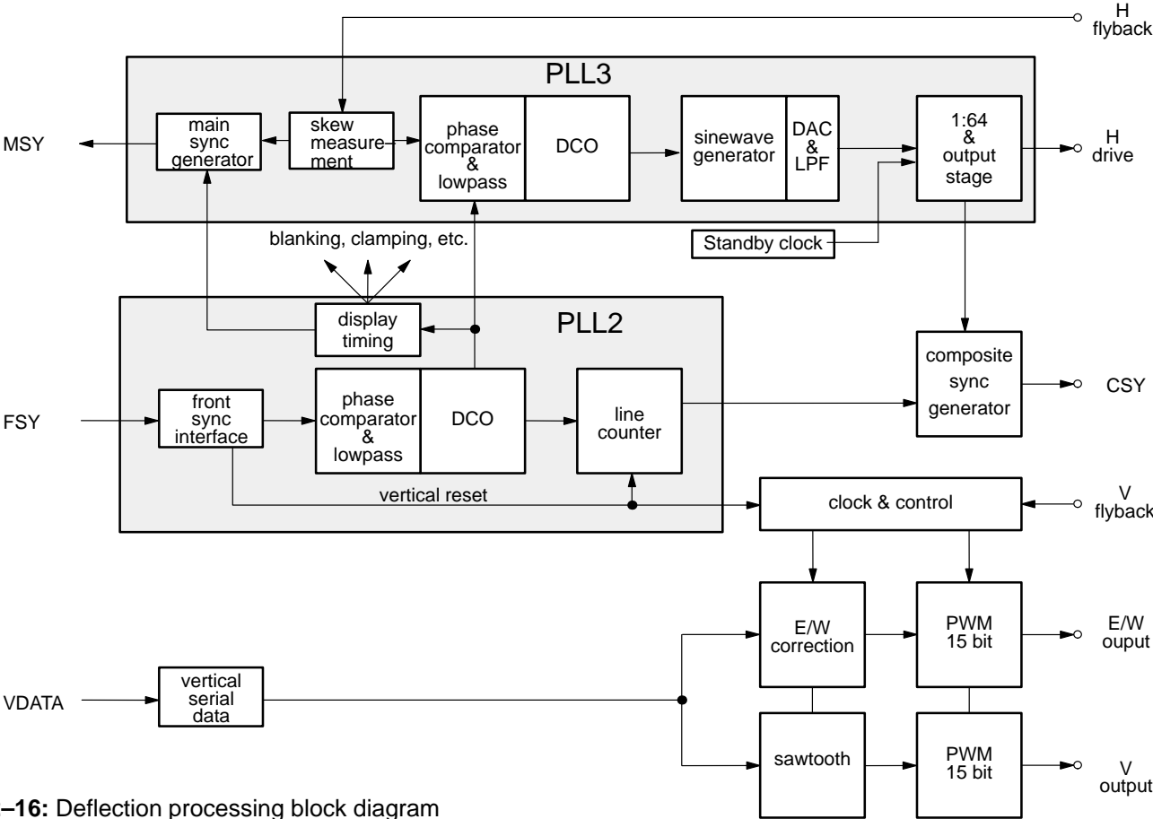
Fig. 2-16: Deflection processing block diagram
