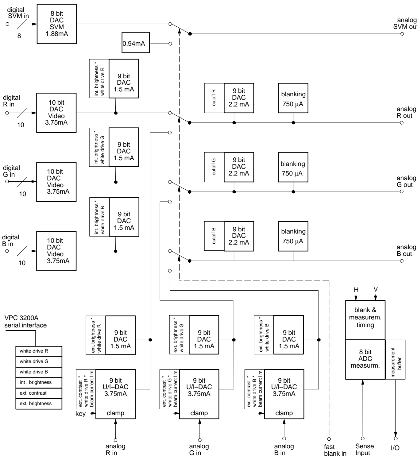
Fig. 2-14:Analog back-end
