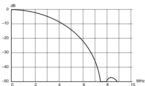
Fig. 2–6:Frequency response of the chroma interpolation filter
