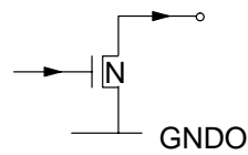
Fig. 4-13: Output pin HOUT
