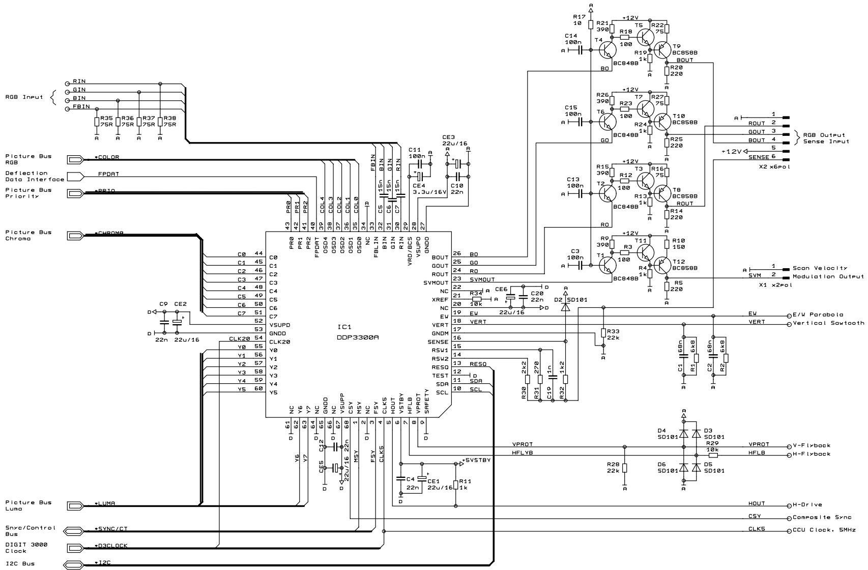
Fig. 5-1: Application diagram
