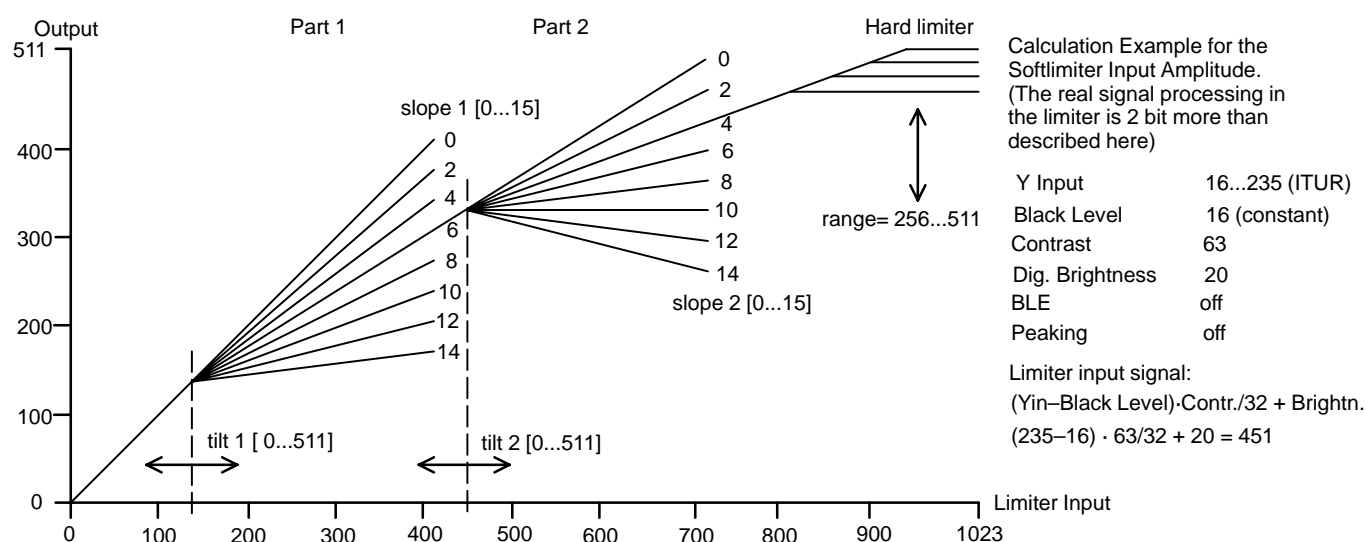
Fig. 2–5:Characteristic of soft limiter a and b and hard limiter
