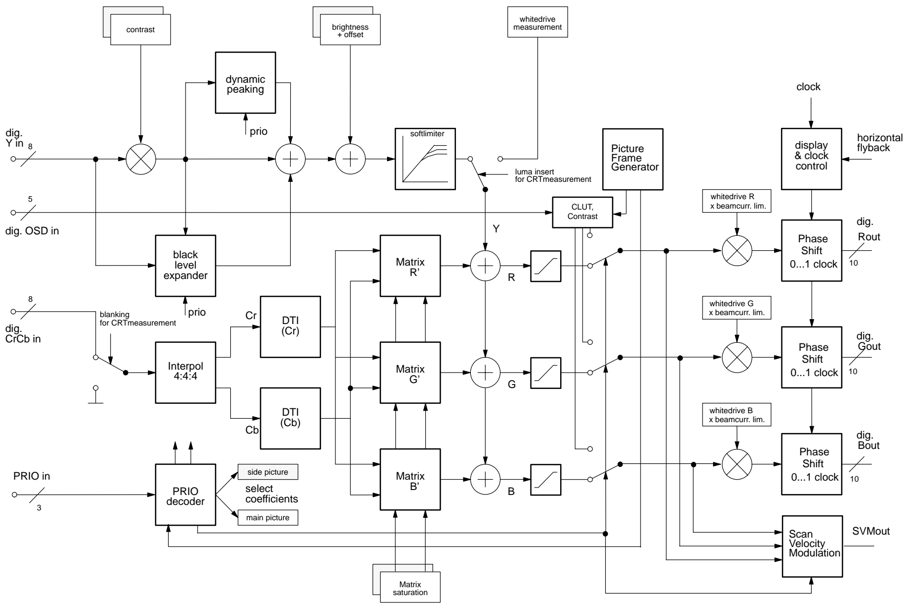
Fig. 2-9:Display part
