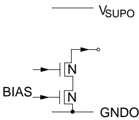
Fig. 4-12: Analog output pins ROUT, GOUT, BOUT, SVMOUT
