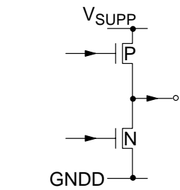
Fig. 4-5: Output pins MSY, CSY
