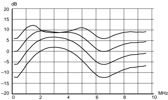
Fig. 2–3:Dynamic peaking frequency response
