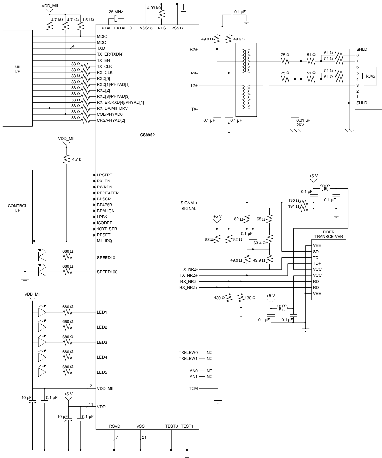
Figure 1. Typical Connection Diagram
