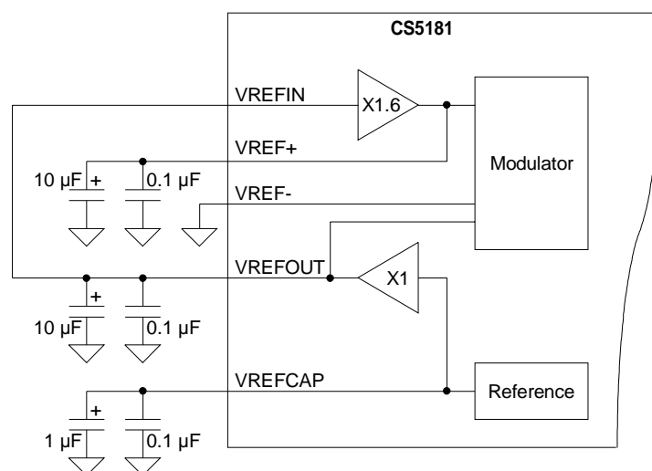
Figure 3. CS5181 connection diagram for using the internal voltage reference.
